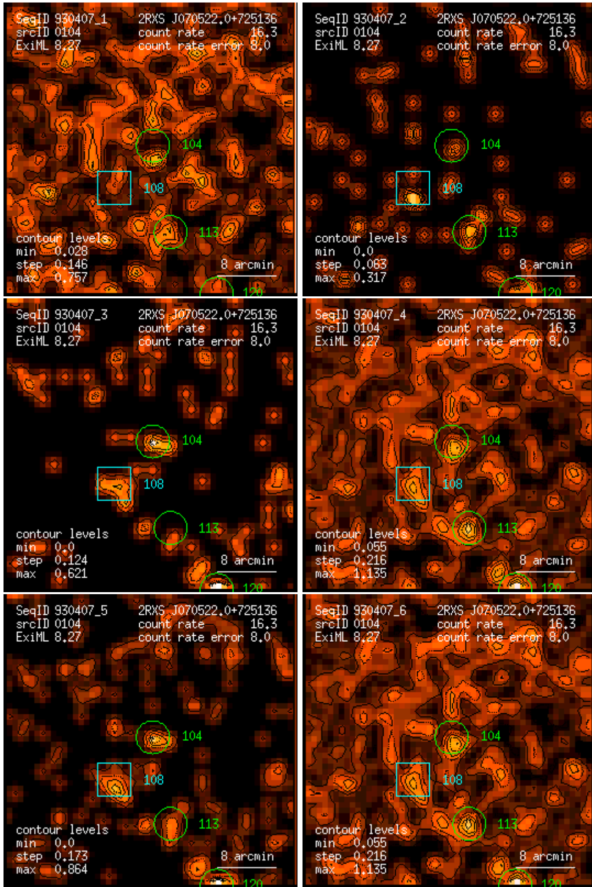
Figure 104: RASS 930407: detection 0104: band rate images, Gaussian filter: (1) PSPC channels 11 – 41, (2) 52 – 90, (3) 91 – 201, (4) 11 – 235, (5) 52 – 201, (6) 11 – 201. Broad band rates in counts/ks. Band rate contour levels in counts/ks/arcmin 2 .
