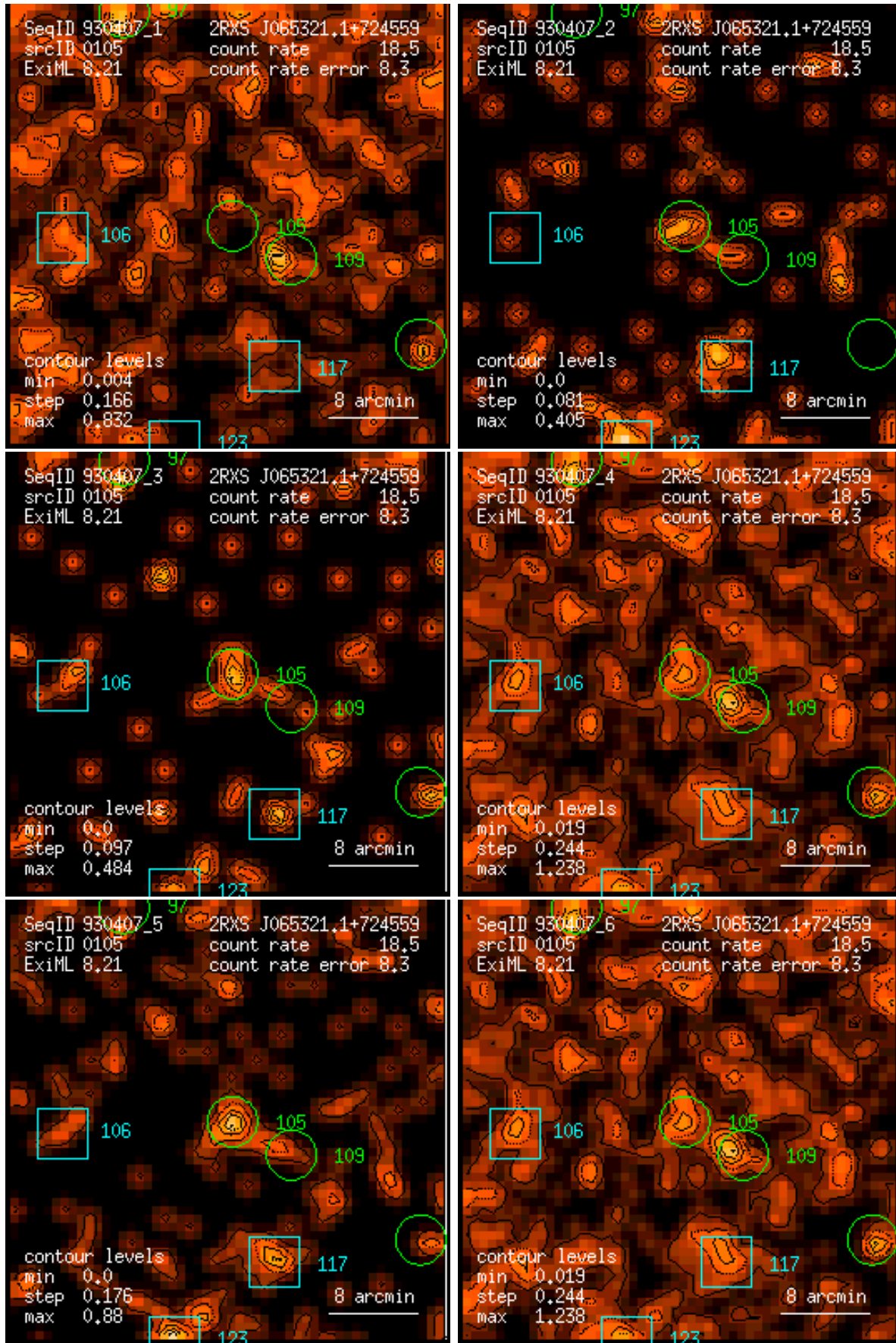
Figure 105: RASS 930407: detection 0105: band rate images, Gaussian filter: (1) PSPC channels 11 – 41, (2) 52 – 90, (3) 91 – 201, (4) 11 – 235, (5) 52 – 201, (6) 11 – 201. Broad band rates in counts/ks. Band rate contour levels in counts/ks/arcmin 2 .
