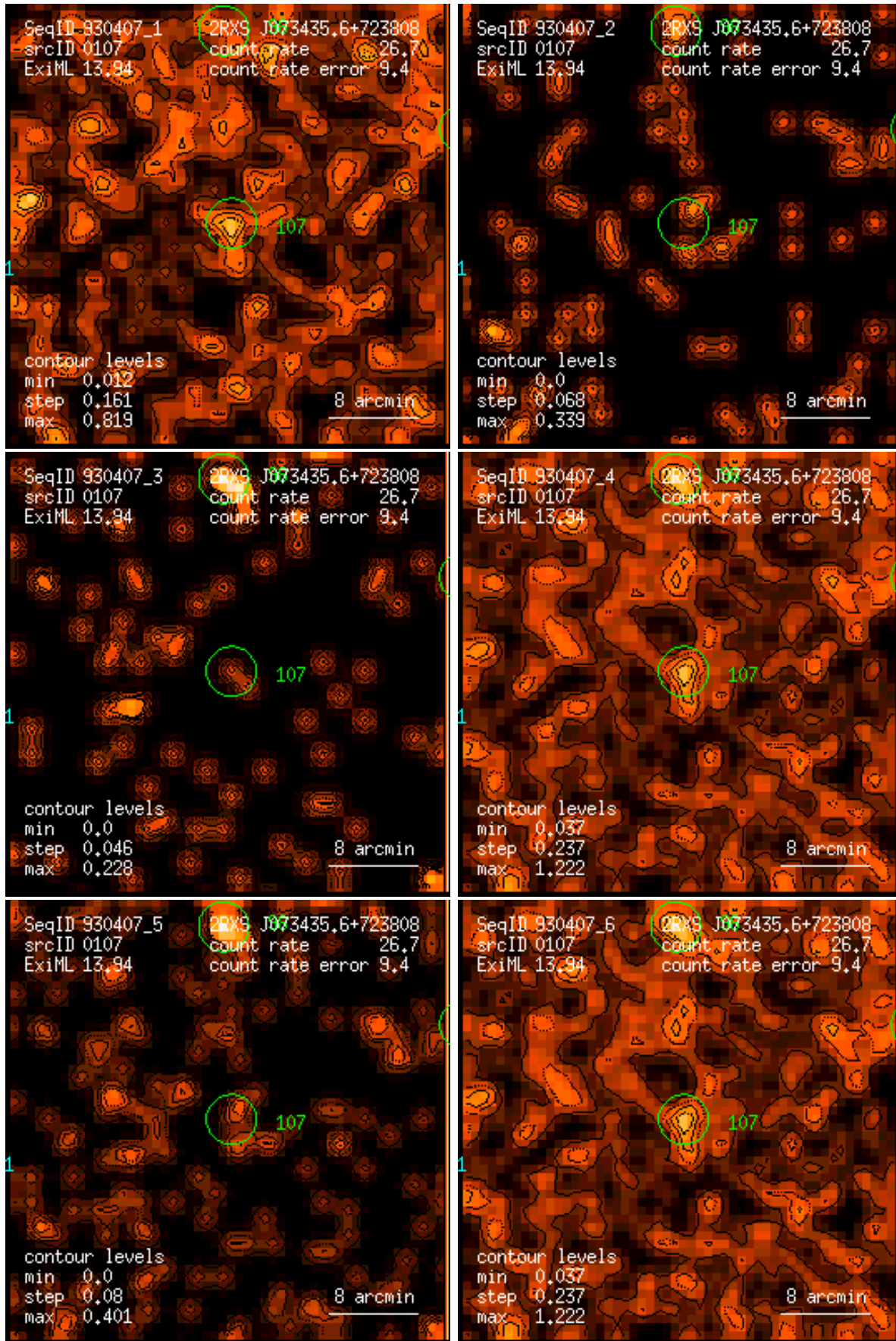
Figure 107: RASS 930407: detection 0107: band rate images, Gaussian filter: (1) PSPC channels 11 – 41, (2) 52 – 90, (3) 91 – 201, (4) 11 – 235, (5) 52 – 201, (6) 11 – 201. Broad band rates in counts/ks. Band rate contour levels in counts/ks/arcmin 2 .
