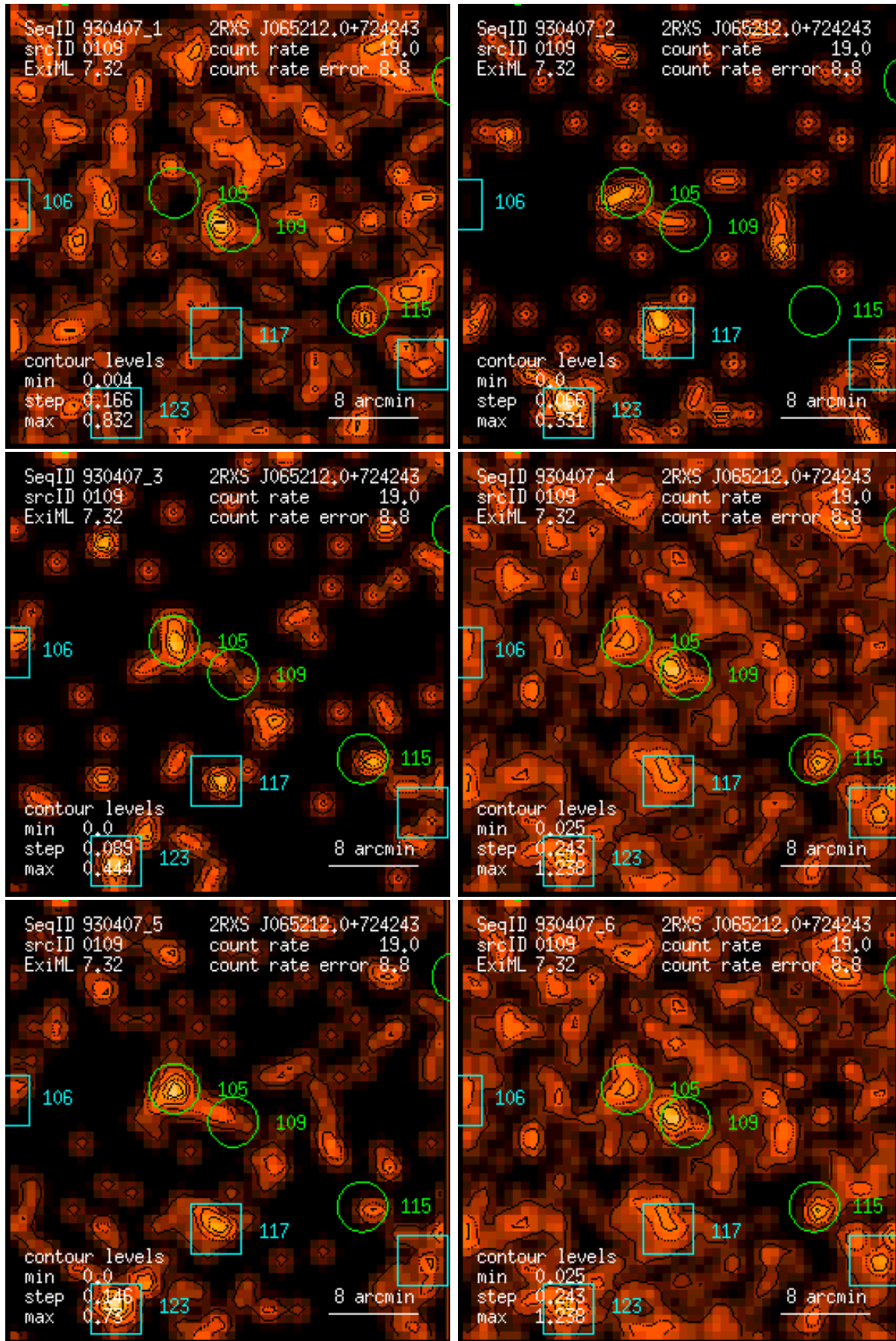
Figure 109: RASS 930407: detection 0109: band rate images, Gaussian filter: (1) PSPC channels 11 – 41, (2) 52 – 90, (3) 91 – 201, (4) 11 – 235, (5) 52 – 201, (6) 11 – 201. Broad band rates in counts/ks. Band rate contour levels in counts/ks/arcmin 2 .
