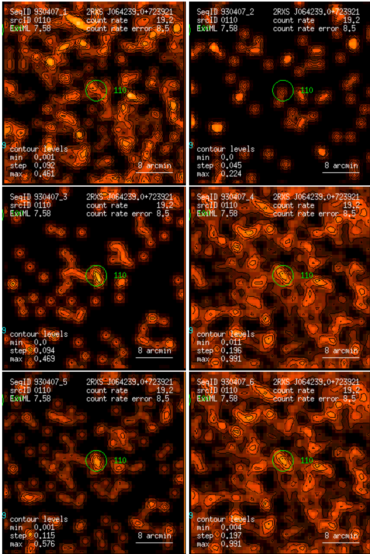
Figure 110: RASS 930407: detection 0110: band rate images, Gaussian filter: (1) PSPC channels 11 – 41, (2) 52 – 90, (3) 91 – 201, (4) 11 – 235, (5) 52 – 201, (6) 11 – 201. Broad band rates in counts/ks. Band rate contour levels in counts/ks/arcmin 2 .
