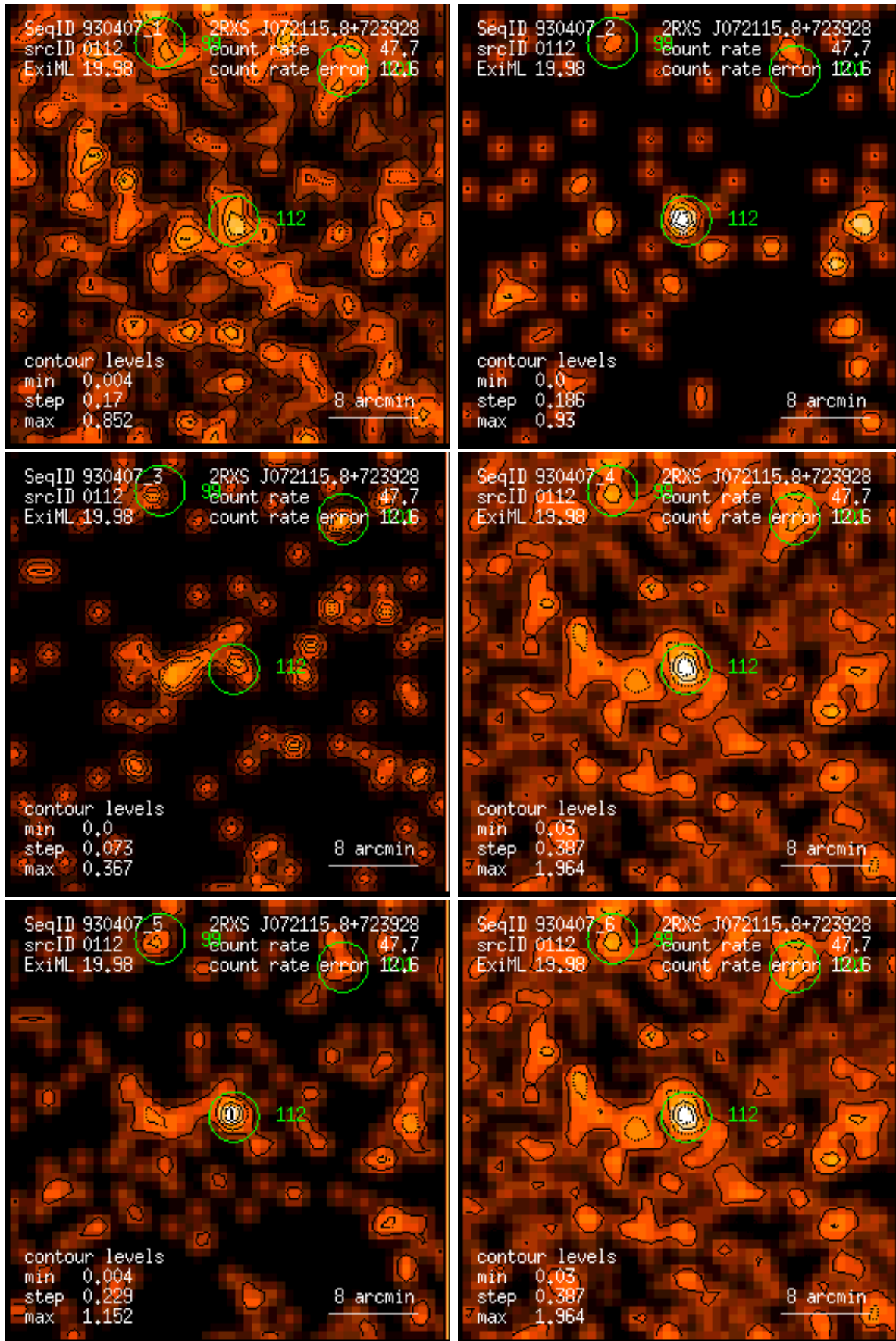
Figure 112: RASS 930407: detection 0112: band rate images, Gaussian filter: (1) PSPC channels 11 – 41, (2) 52 – 90, (3) 91 – 201, (4) 11 – 235, (5) 52 – 201, (6) 11 – 201. Broad band rates in counts/ks. Band rate contour levels in counts/ks/arcmin 2 .
