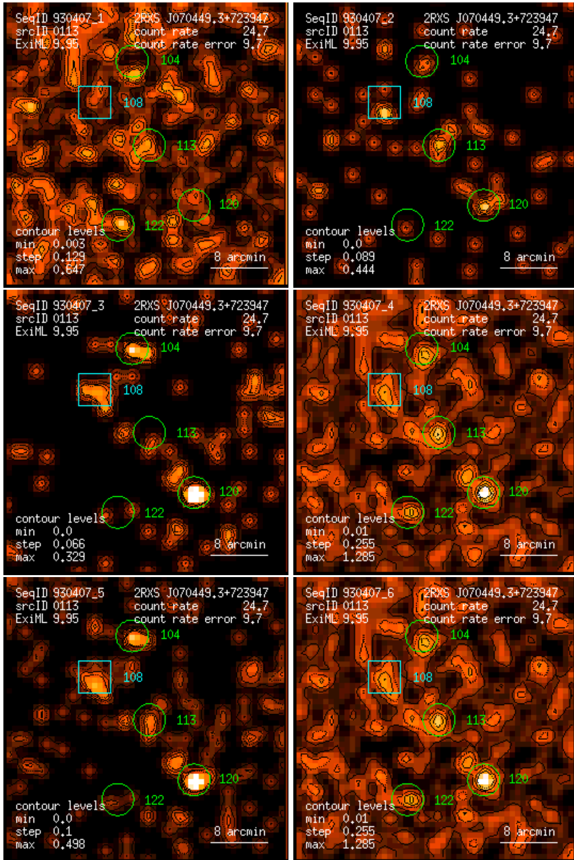
Figure 113: RASS 930407: detection 0113: band rate images, Gaussian filter: (1) PSPC channels 11 – 41, (2) 52 – 90, (3) 91 – 201, (4) 11 – 235, (5) 52 – 201, (6) 11 – 201. Broad band rates in counts/ks. Band rate contour levels in counts/ks/arcmin 2 .
