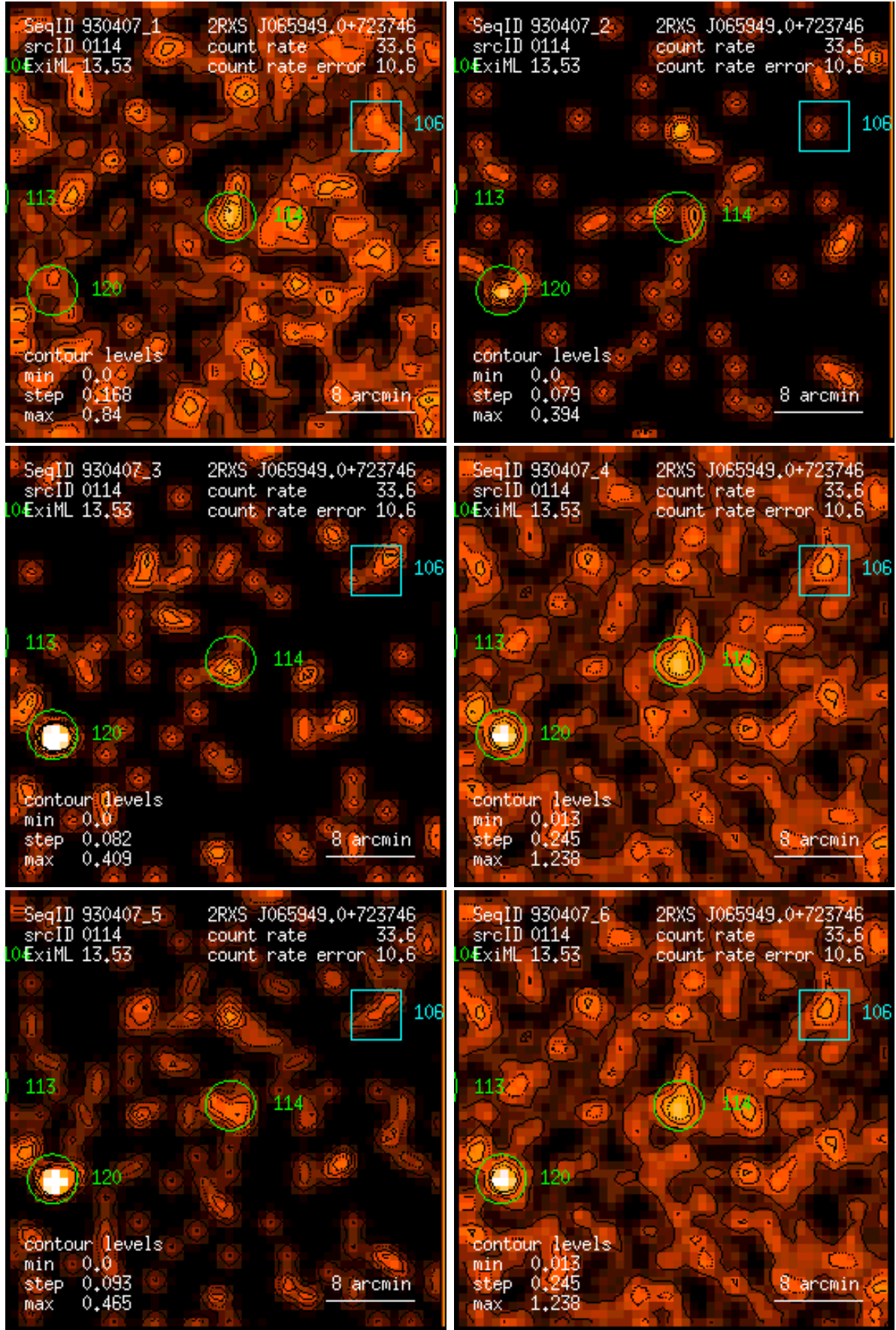
Figure 114: RASS 930407: detection 0114: band rate images, Gaussian filter: (1) PSPC channels 11 – 41, (2) 52 – 90, (3) 91 – 201, (4) 11 – 235, (5) 52 – 201, (6) 11 – 201. Broad band rates in counts/ks. Band rate contour levels in counts/ks/arcmin 2 .
