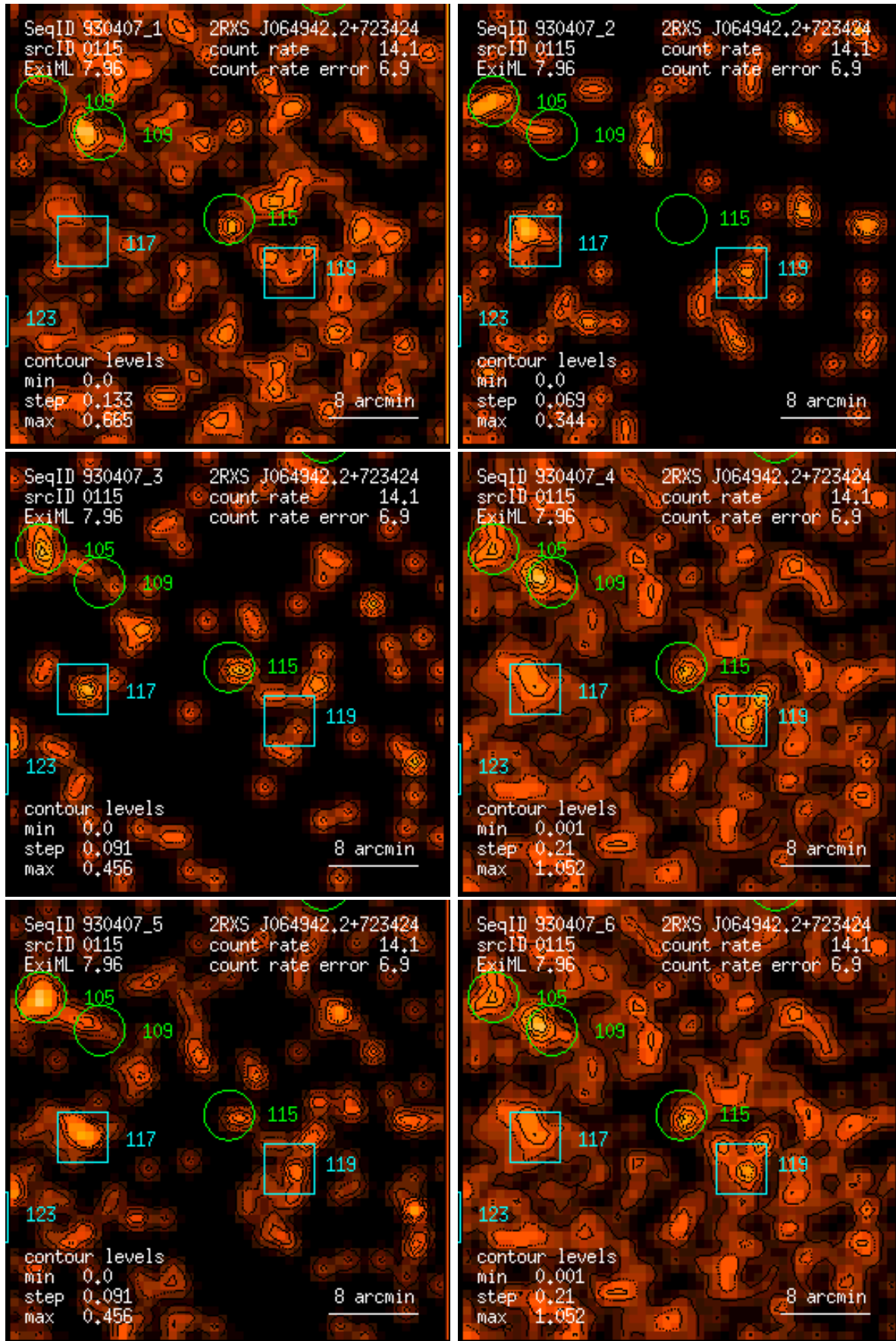
Figure 115: RASS 930407: detection 0115: band rate images, Gaussian filter: (1) PSPC channels 11 – 41, (2) 52 – 90, (3) 91 – 201, (4) 11 – 235, (5) 52 – 201, (6) 11 – 201. Broad band rates in counts/ks. Band rate contour levels in counts/ks/arcmin 2 .
