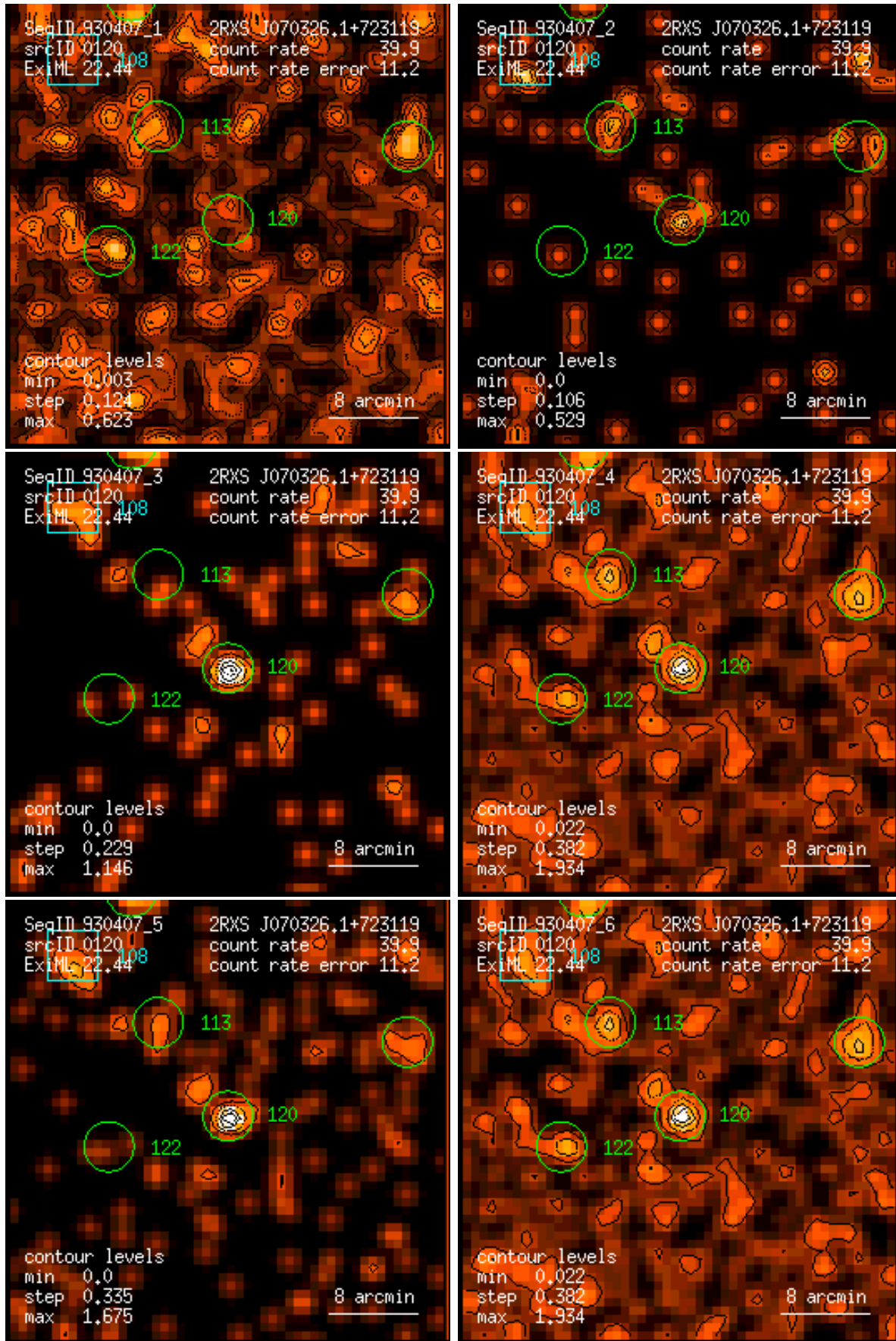
Figure 120: RASS 930407: detection 0120: band rate images, Gaussian filter: (1) PSPC channels 11 – 41, (2) 52 – 90, (3) 91 – 201, (4) 11 – 235, (5) 52 – 201, (6) 11 – 201. Broad band rates in counts/ks. Band rate contour levels in counts/ks/arcmin 2 .
