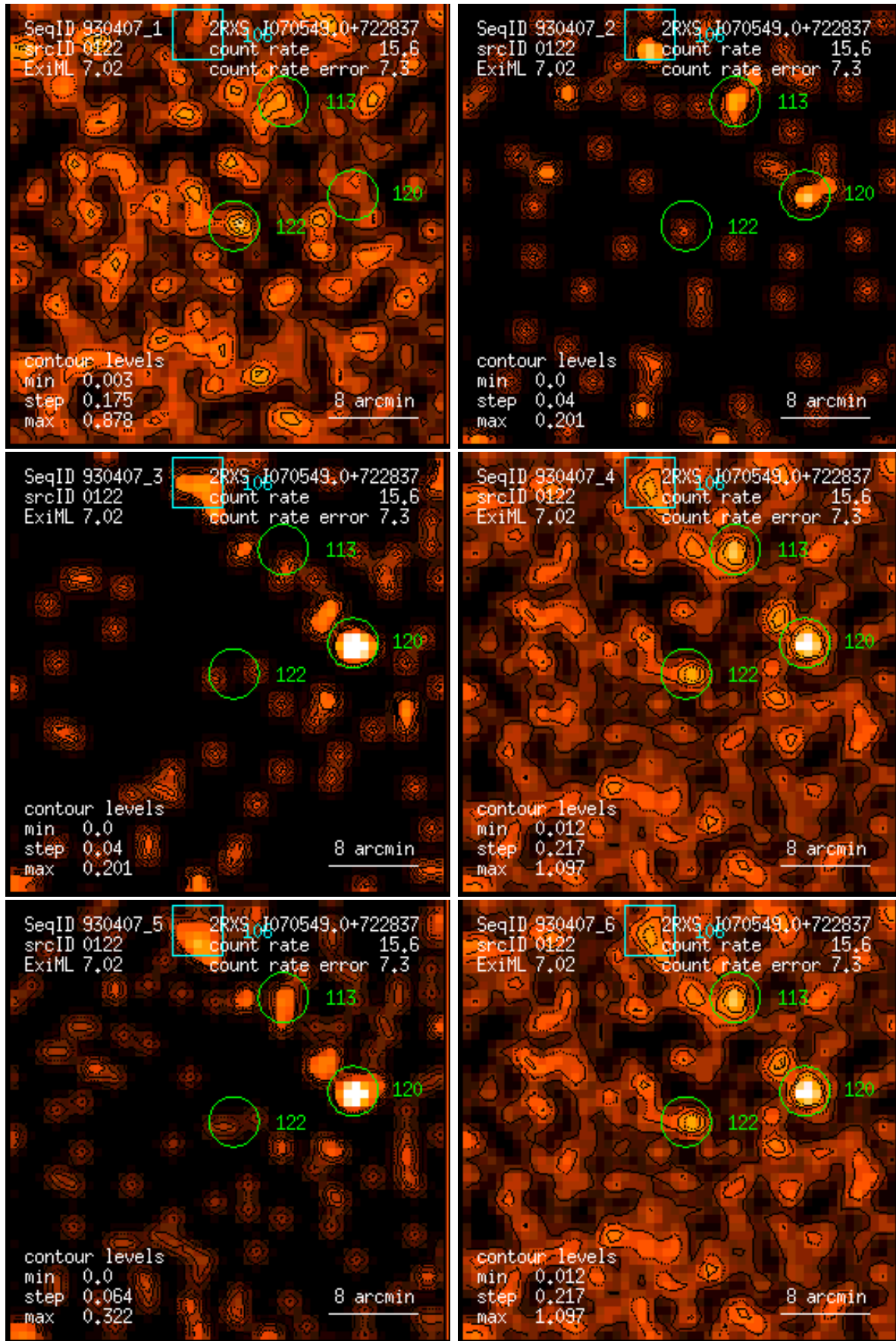
Figure 122: RASS 930407: detection 0122: band rate images, Gaussian filter: (1) PSPC channels 11 – 41, (2) 52 – 90, (3) 91 – 201, (4) 11 – 235, (5) 52 – 201, (6) 11 – 201. Broad band rates in counts/ks. Band rate contour levels in counts/ks/arcmin 2 .
