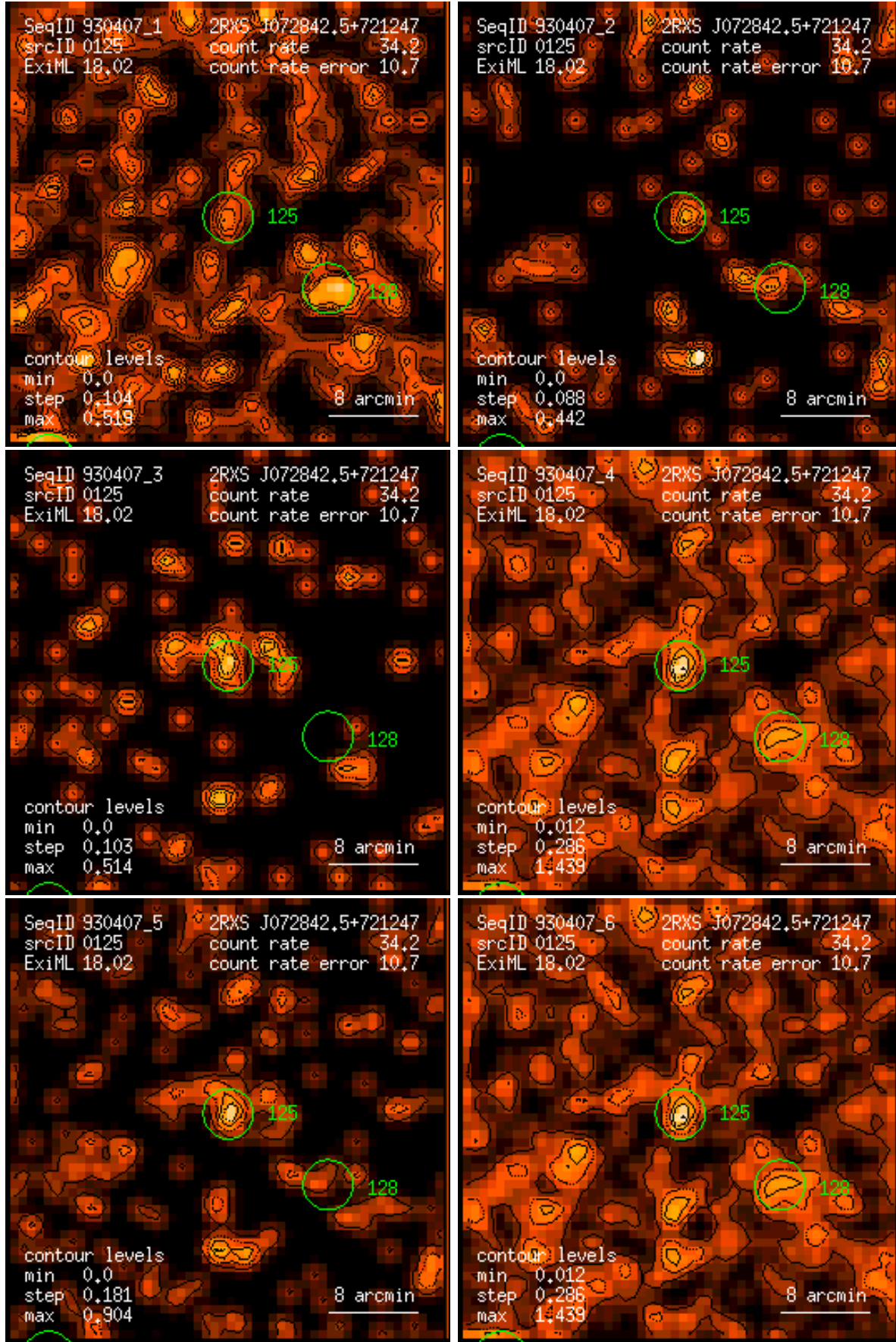
Figure 125: RASS 930407: detection 0125: band rate images, Gaussian filter: (1) PSPC channels 11 – 41, (2) 52 – 90, (3) 91 – 201, (4) 11 – 235, (5) 52 – 201, (6) 11 – 201. Broad band rates in counts/ks. Band rate contour levels in counts/ks/arcmin 2 .
