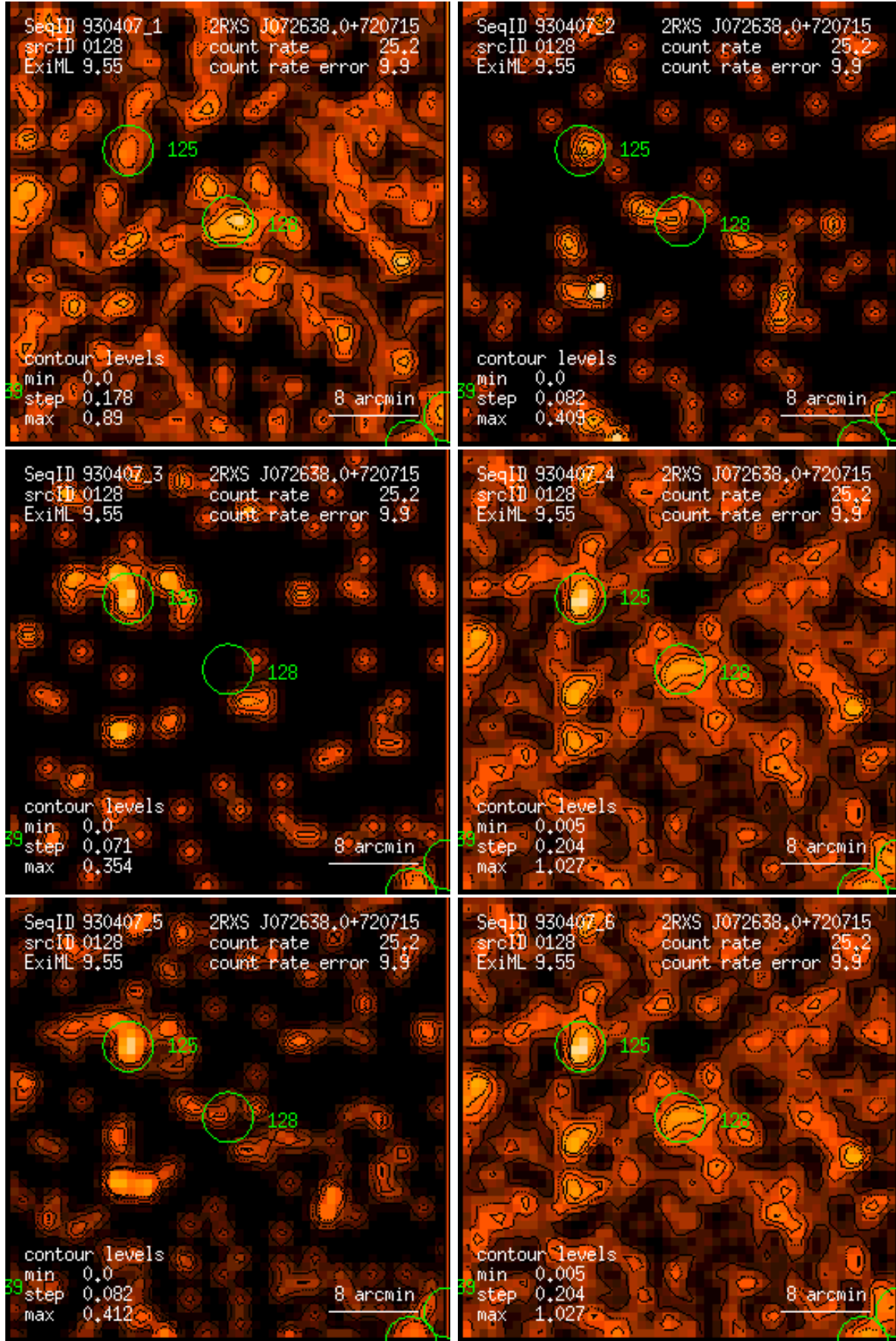
Figure 128: RASS 930407: detection 0128: band rate images, Gaussian filter: (1) PSPC channels 11 – 41, (2) 52 – 90, (3) 91 – 201, (4) 11 – 235, (5) 52 – 201, (6) 11 – 201. Broad band rates in counts/ks. Band rate contour levels in counts/ks/arcmin 2 .
