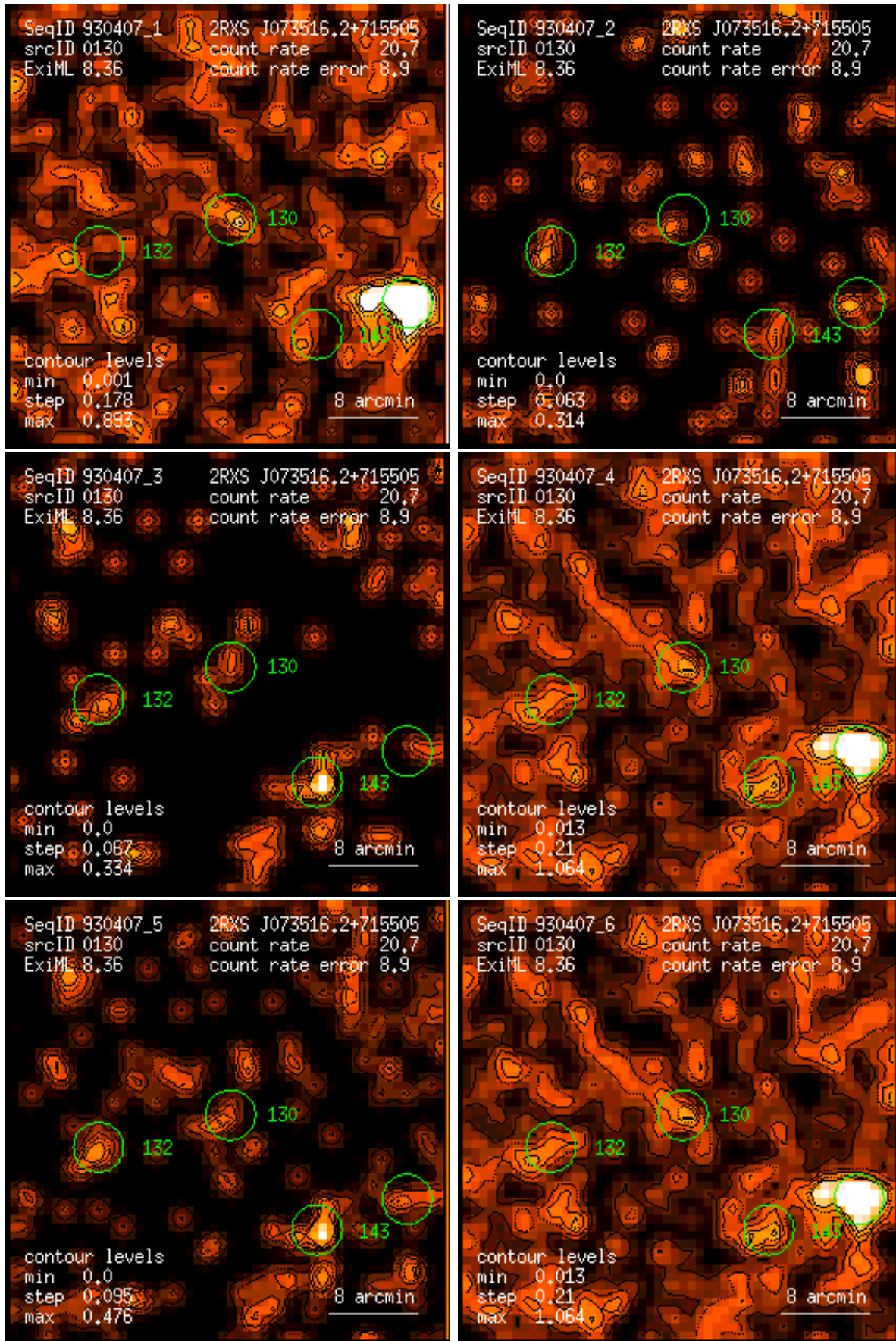
Figure 130: RASS 930407: detection 0130: band rate images, Gaussian filter: (1) PSPC channels 11 – 41, (2) 52 – 90, (3) 91 – 201, (4) 11 – 235, (5) 52 – 201, (6) 11 – 201. Broad band rates in counts/ks. Band rate contour levels in counts/ks/arcmin 2 .
