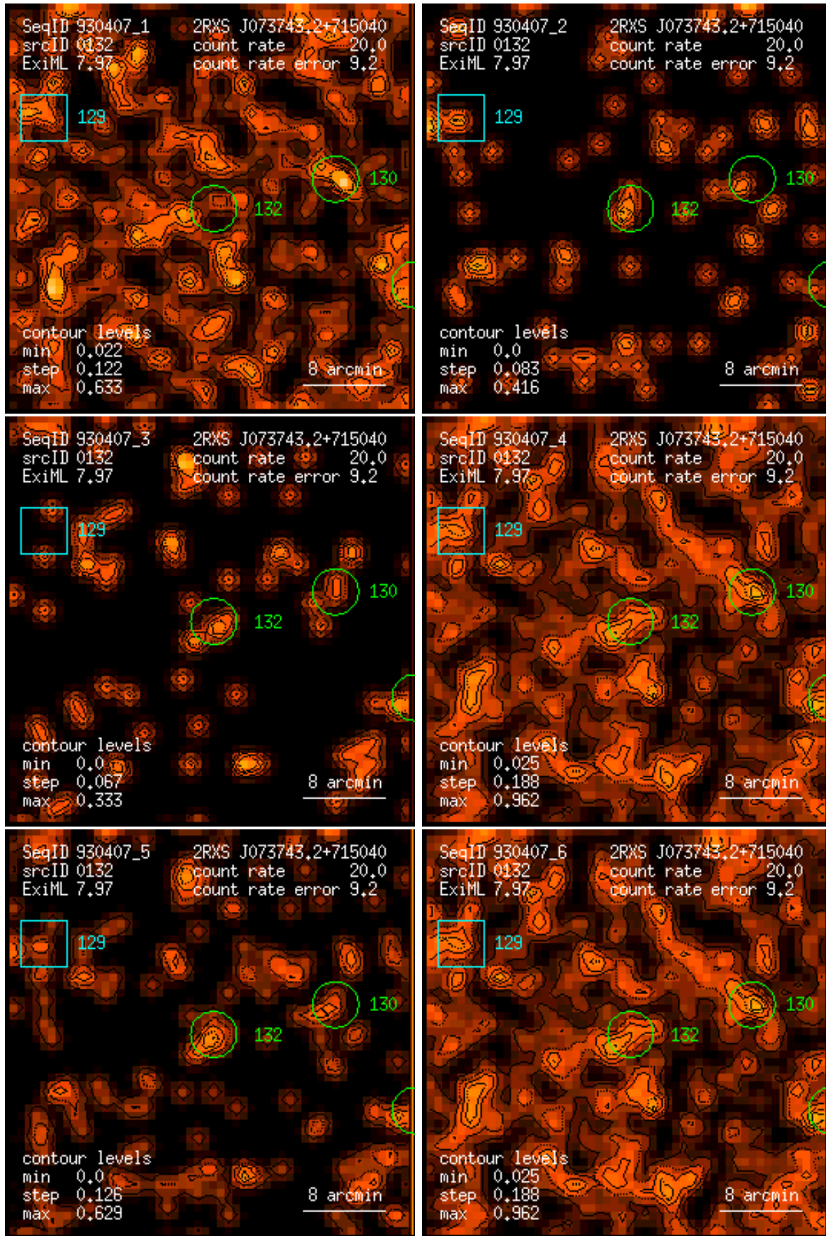
Figure 132: RASS 930407: detection 0132: band rate images, Gaussian filter: (1) PSPC channels 11 – 41, (2) 52 – 90, (3) 91 – 201, (4) 11 – 235, (5) 52 – 201, (6) 11 – 201. Broad band rates in counts/ks. Band rate contour levels in counts/ks/arcmin 2 .
