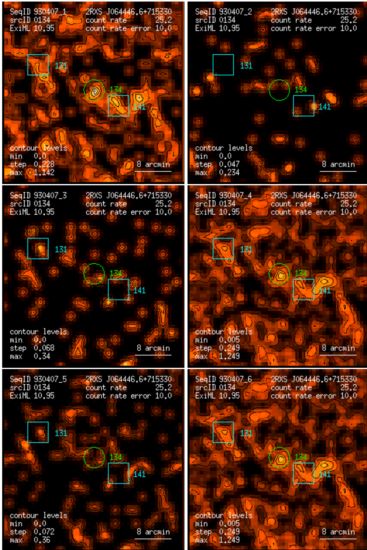
Figure 134: RASS 930407: detection 0134: band rate images, Gaussian filter: (1) PSPC channels 11 – 41, (2) 52 – 90, (3) 91 – 201, (4) 11 – 235, (5) 52 – 201, (6) 11 – 201. Broad band rates in counts/ks. Band rate contour levels in counts/ks/arcmin 2 .
