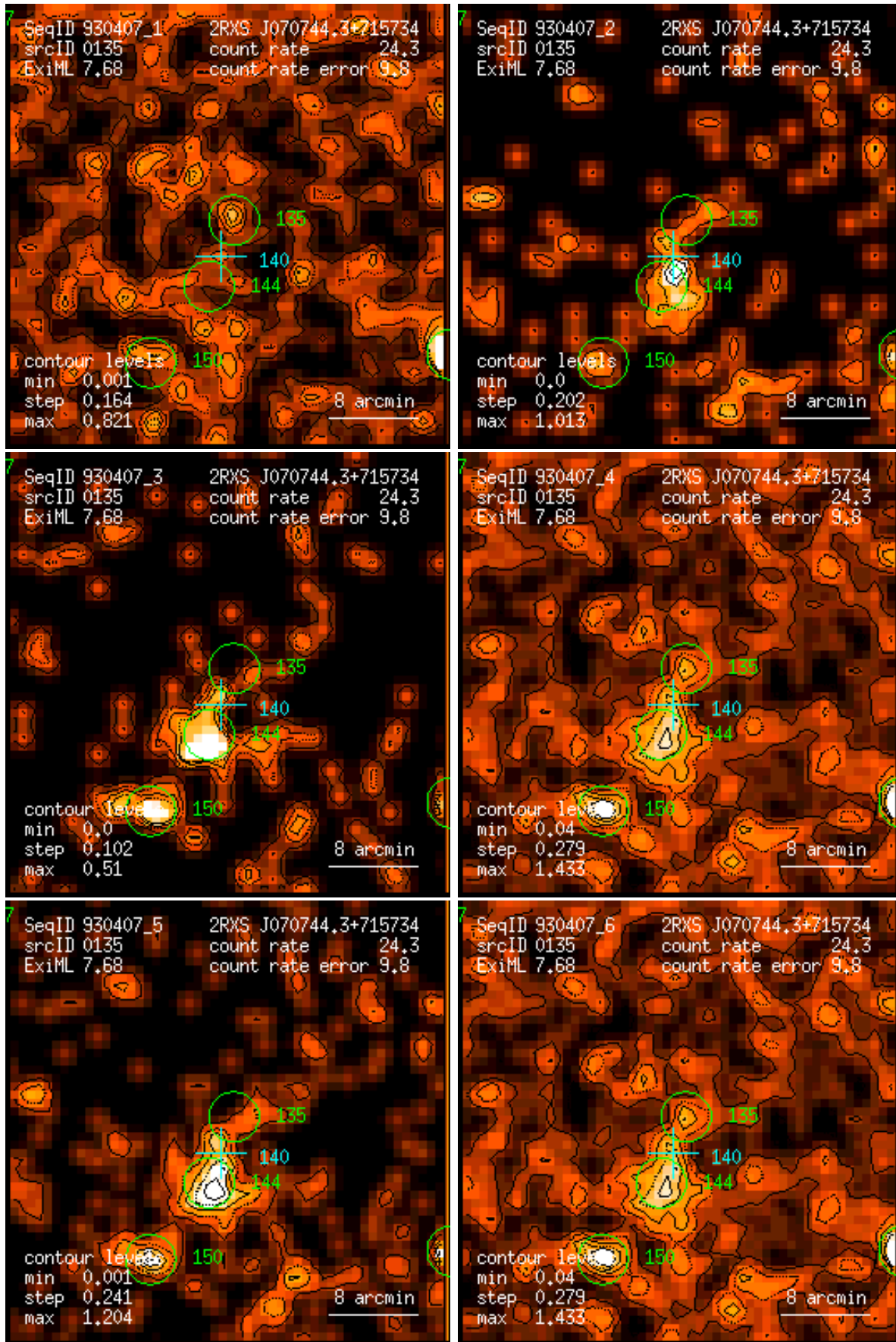
Figure 135: RASS 930407: detection 0135: band rate images, Gaussian filter: (1) PSPC channels 11 – 41, (2) 52 – 90, (3) 91 – 201, (4) 11 – 235, (5) 52 – 201, (6) 11 – 201. Broad band rates in counts/ks. Band rate contour levels in counts/ks/arcmin 2 .
