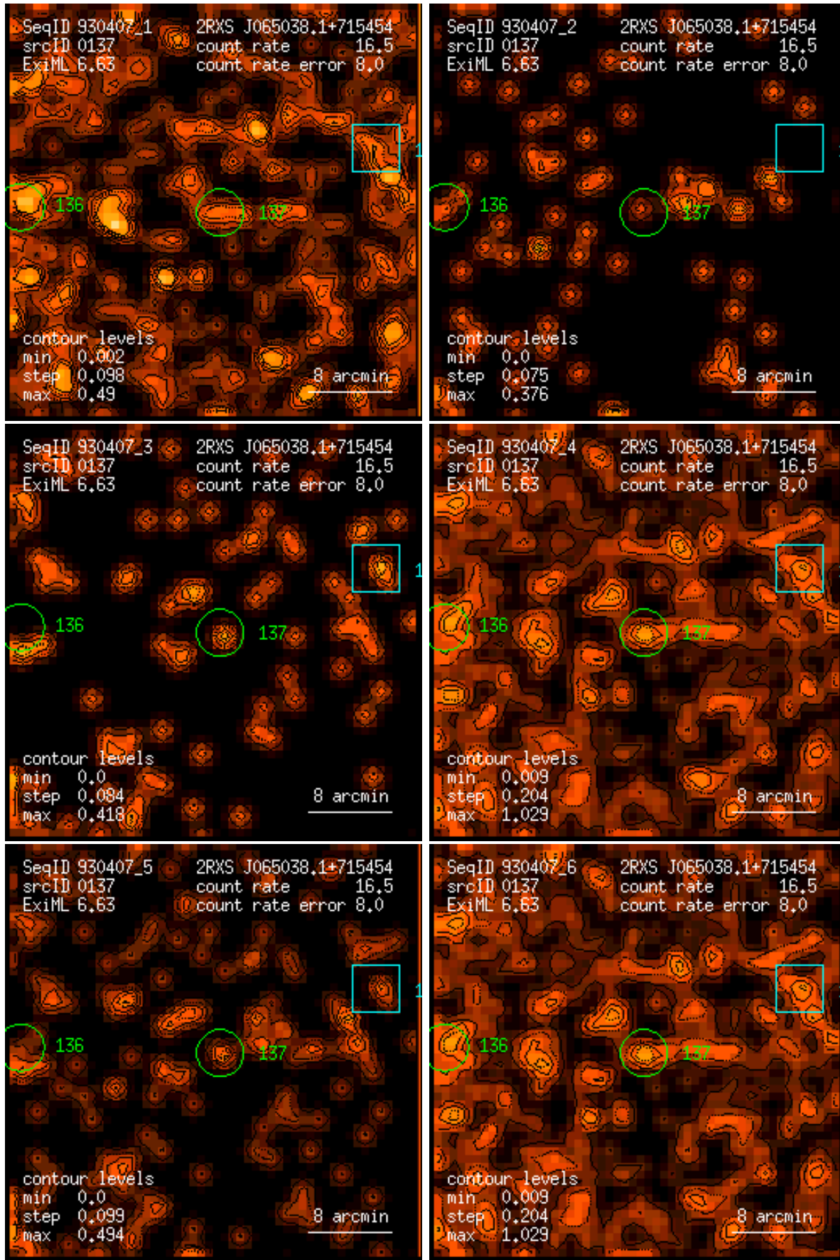
Figure 137: RASS 930407: detection 0137: band rate images, Gaussian filter: (1) PSPC channels 11 – 41, (2) 52 – 90, (3) 91 – 201, (4) 11 – 235, (5) 52 – 201, (6) 11 – 201. Broad band rates in counts/ks. Band rate contour levels in counts/ks/arcmin 2 .
