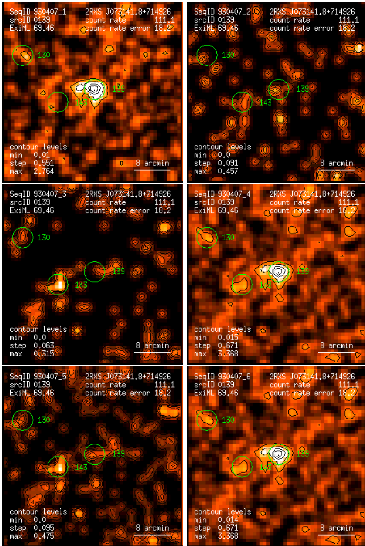
Figure 139: RASS 930407: detection 0139: band rate images, Gaussian filter: (1) PSPC channels 11 – 41, (2) 52 – 90, (3) 91 – 201, (4) 11 – 235, (5) 52 – 201, (6) 11 – 201. Broad band rates in counts/ks. Band rate contour levels in counts/ks/arcmin 2 .
