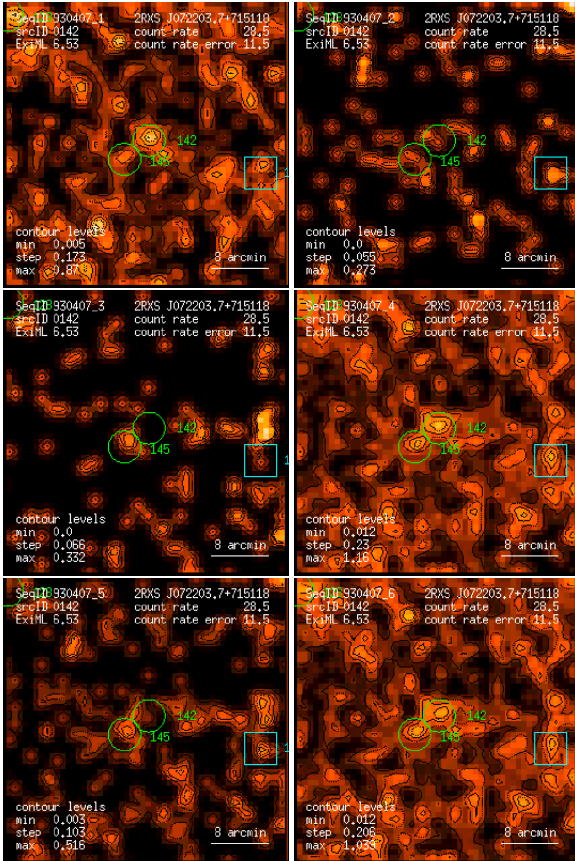
Figure 142: RASS 930407: detection 0142: band rate images, Gaussian filter: (1) PSPC channels 11 – 41, (2) 52 – 90, (3) 91 – 201, (4) 11 – 235, (5) 52 – 201, (6) 11 – 201. Broad band rates in counts/ks. Band rate contour levels in counts/ks/arcmin 2 .
