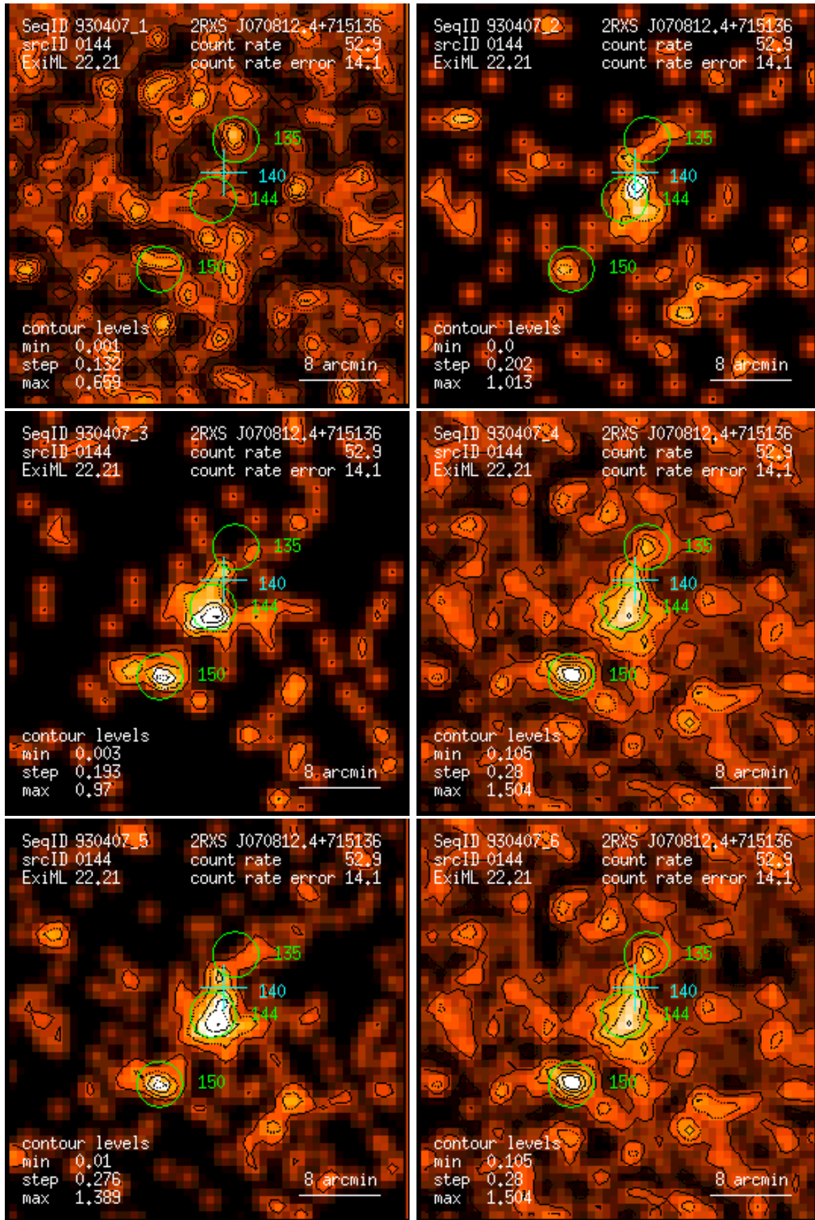
Figure 144: RASS 930407: detection 0144: band rate images, Gaussian filter: (1) PSPC channels 11 – 41, (2) 52 – 90, (3) 91 – 201, (4) 11 – 235, (5) 52 – 201, (6) 11 – 201. Broad band rates in counts/ks. Band rate contour levels in counts/ks/arcmin 2 .
