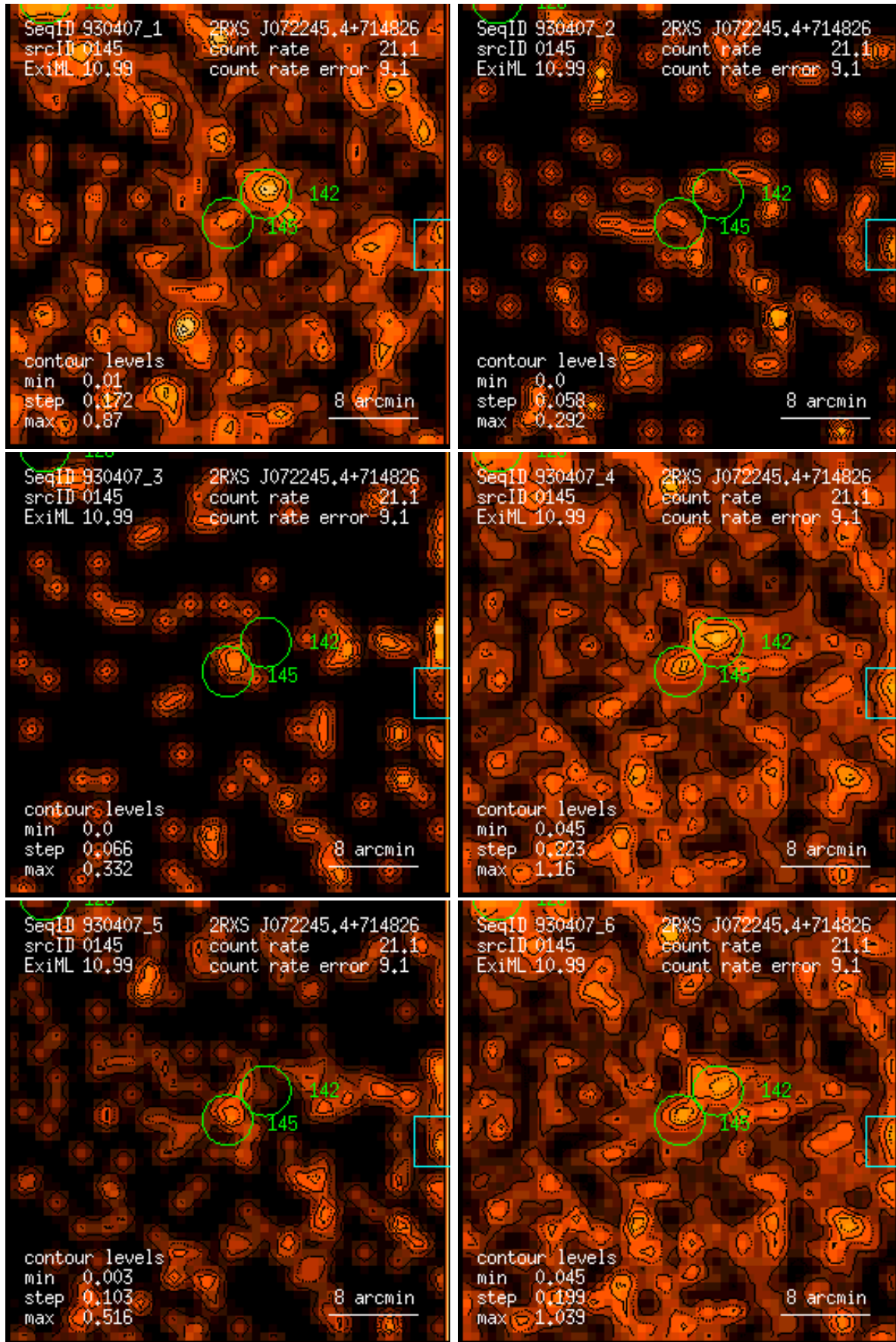
Figure 145: RASS 930407: detection 0145: band rate images, Gaussian filter: (1) PSPC channels 11 – 41, (2) 52 – 90, (3) 91 – 201, (4) 11 – 235, (5) 52 – 201, (6) 11 – 201. Broad band rates in counts/ks. Band rate contour levels in counts/ks/arcmin 2 .
