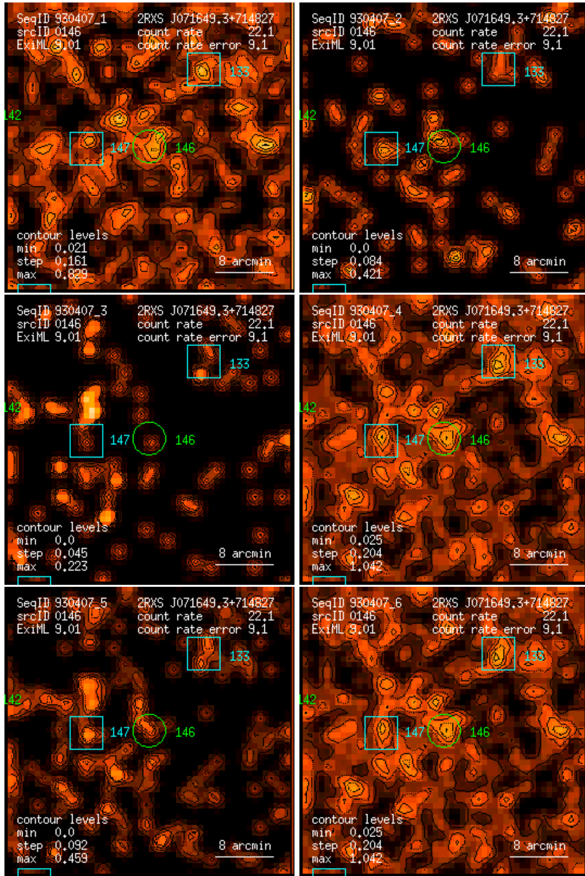
Figure 146: RASS 930407: detection 0146: band rate images, Gaussian filter: (1) PSPC channels 11 – 41, (2) 52 – 90, (3) 91 – 201, (4) 11 – 235, (5) 52 – 201, (6) 11 – 201. Broad band rates in counts/ks. Band rate contour levels in counts/ks/arcmin 2 .
