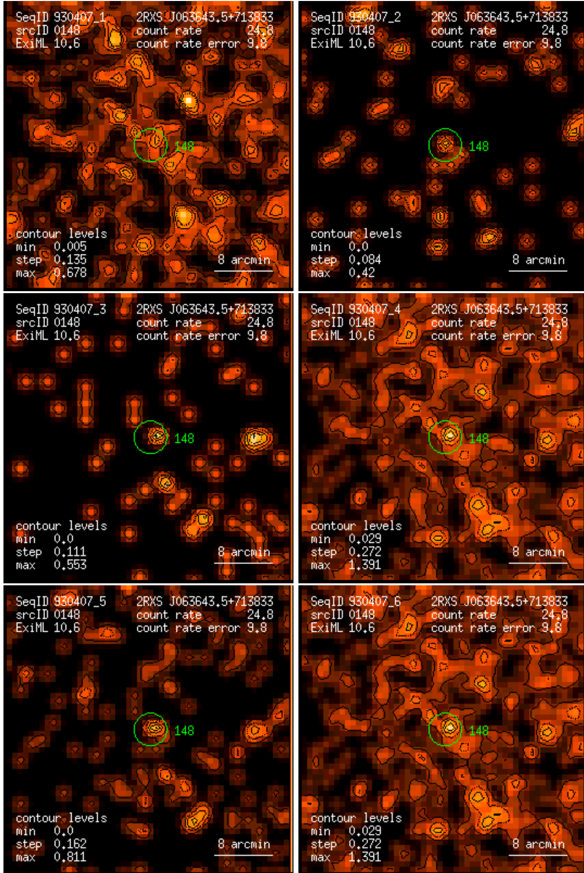
Figure 148: RASS 930407: detection 0148: band rate images, Gaussian filter: (1) PSPC channels 11 – 41, (2) 52 – 90, (3) 91 – 201, (4) 11 – 235, (5) 52 – 201, (6) 11 – 201. Broad band rates in counts/ks. Band rate contour levels in counts/ks/arcmin 2 .
