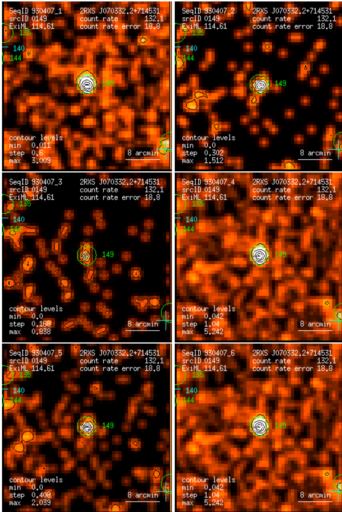
Figure 149: RASS 930407: detection 0149: band rate images, Gaussian filter: (1) PSPC channels 11 – 41, (2) 52 – 90, (3) 91 – 201, (4) 11 – 235, (5) 52 – 201, (6) 11 – 201. Broad band rates in counts/ks. Band rate contour levels in counts/ks/arcmin 2 .
