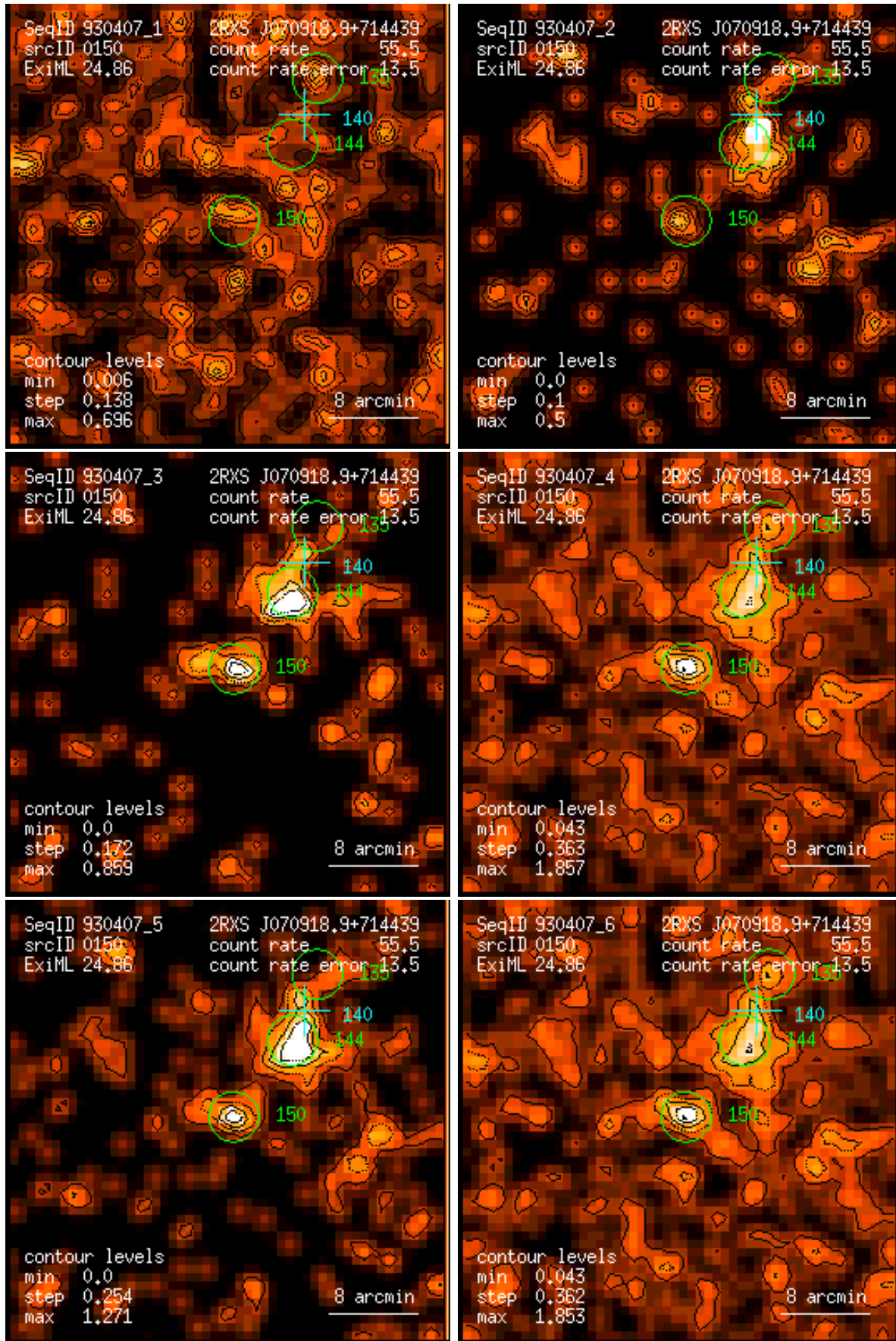
Figure 150: RASS 930407: detection 0150: band rate images, Gaussian filter: (1) PSPC channels 11 – 41, (2) 52 – 90, (3) 91 – 201, (4) 11 – 235, (5) 52 – 201, (6) 11 – 201. Broad band rates in counts/ks. Band rate contour levels in counts/ks/arcmin 2 .
