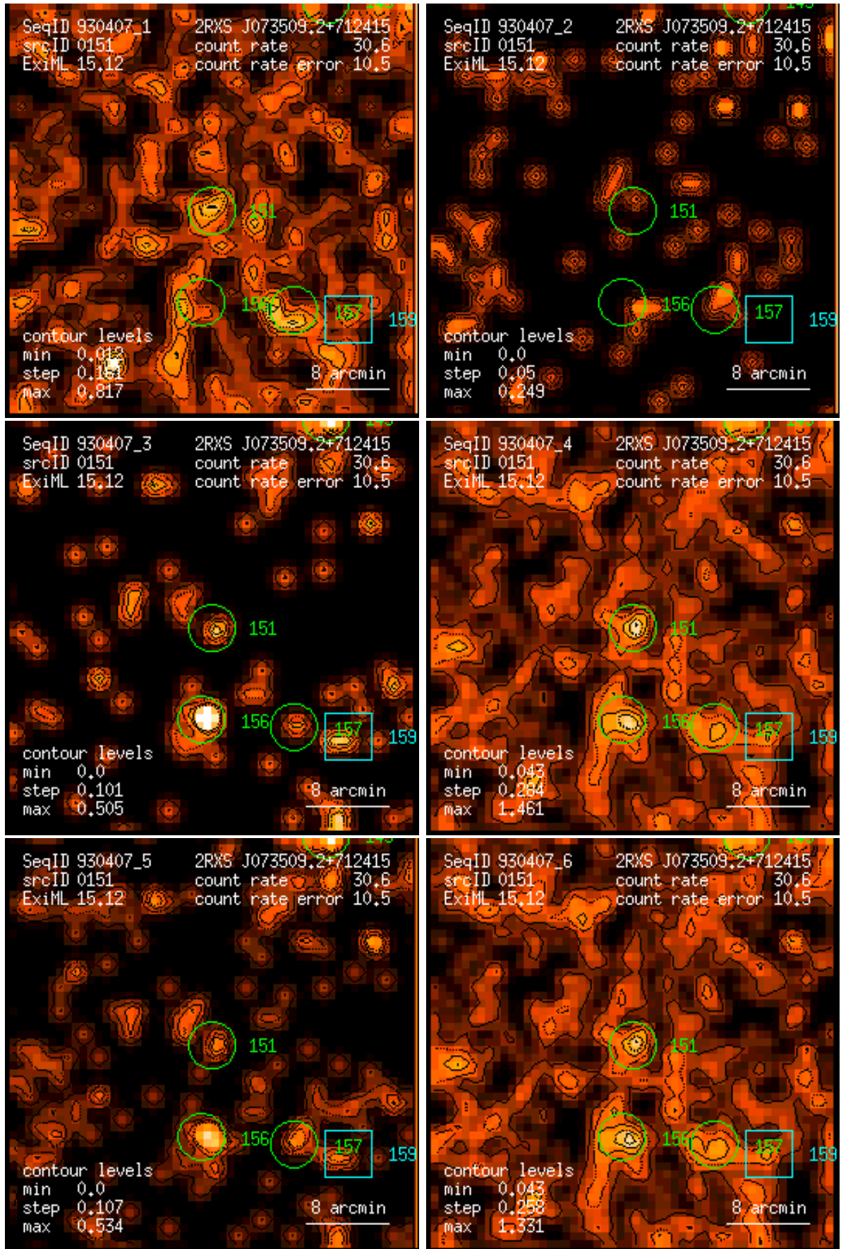
Figure 151: RASS 930407: detection 0151: band rate images, Gaussian filter: (1) PSPC channels 11 – 41, (2) 52 – 90, (3) 91 – 201, (4) 11 – 235, (5) 52 – 201, (6) 11 – 201. Broad band rates in counts/ks. Band rate contour levels in counts/ks/arcmin 2 .
