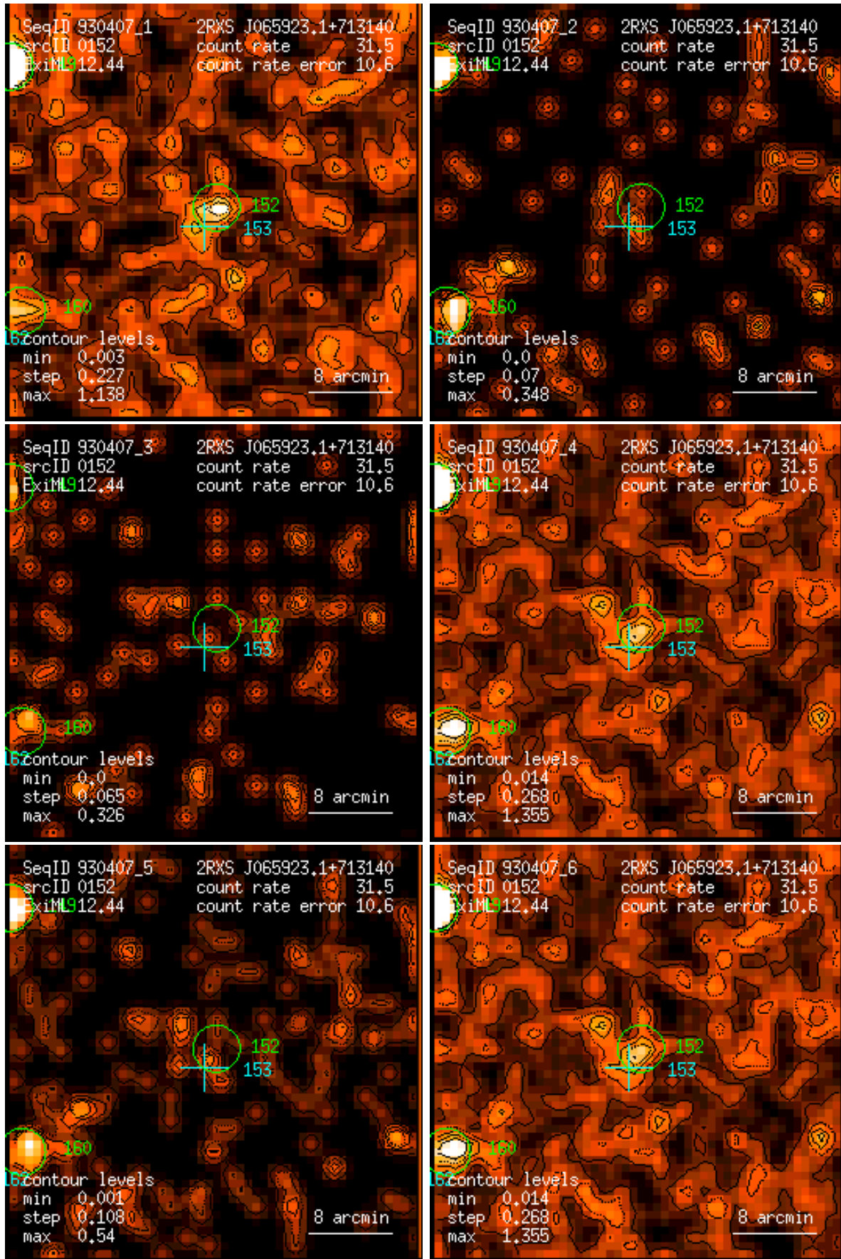
Figure 152: RASS 930407: detection 0152: band rate images, Gaussian filter: (1) PSPC channels 11 – 41, (2) 52 – 90, (3) 91 – 201, (4) 11 – 235, (5) 52 – 201, (6) 11 – 201. Broad band rates in counts/ks. Band rate contour levels in counts/ks/arcmin 2 .
