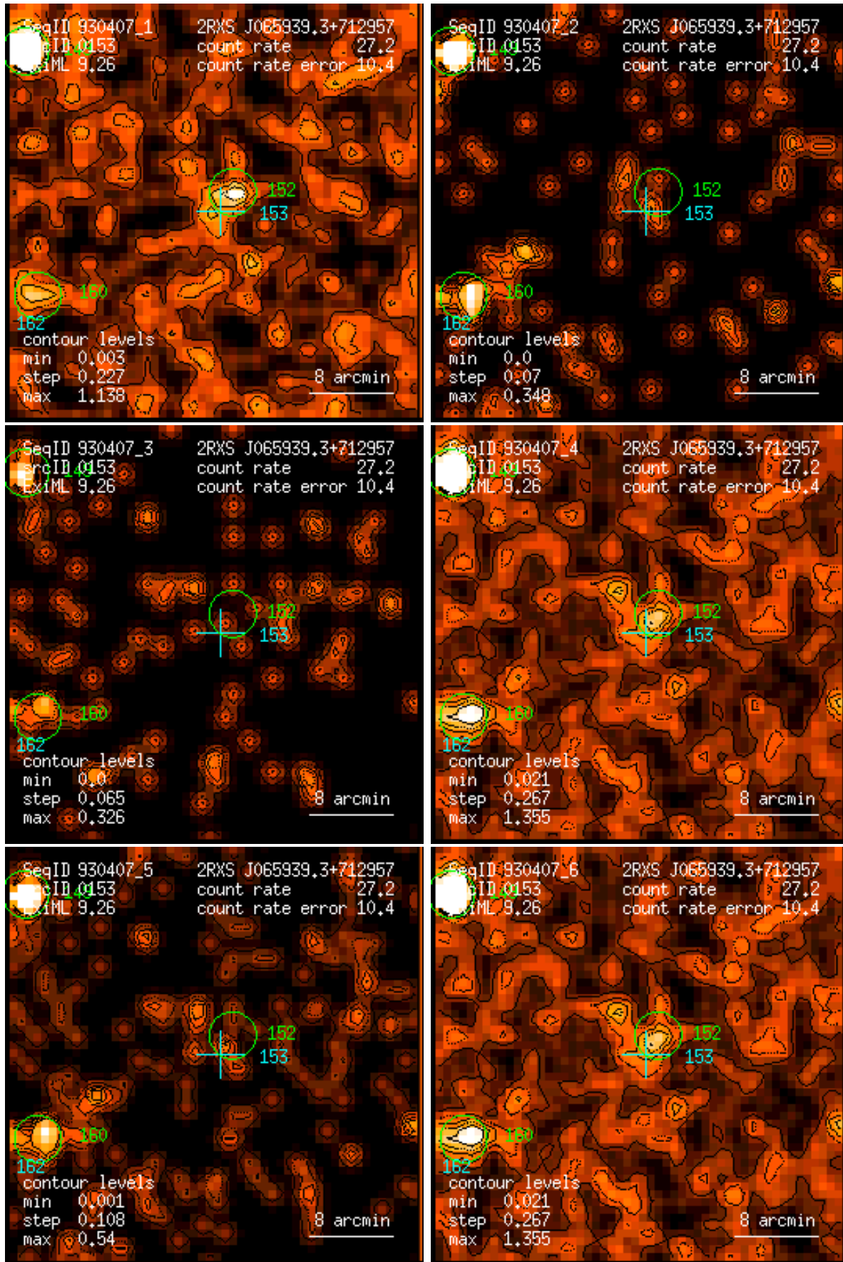
Figure 153: RASS 930407: detection 0153: band rate images, Gaussian filter: (1) PSPC channels 11 – 41, (2) 52 – 90, (3) 91 – 201, (4) 11 – 235, (5) 52 – 201, (6) 11 – 201. Broad band rates in counts/ks. Band rate contour levels in counts/ks/arcmin 2 .
