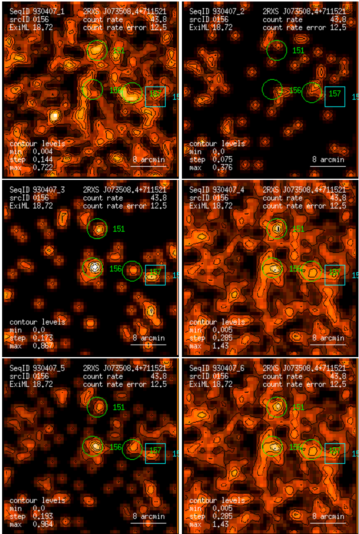
Figure 156: RASS 930407: detection 0156: band rate images, Gaussian filter: (1) PSPC channels 11 – 41, (2) 52 – 90, (3) 91 – 201, (4) 11 – 235, (5) 52 – 201, (6) 11 – 201. Broad band rates in counts/ks. Band rate contour levels in counts/ks/arcmin 2 .
