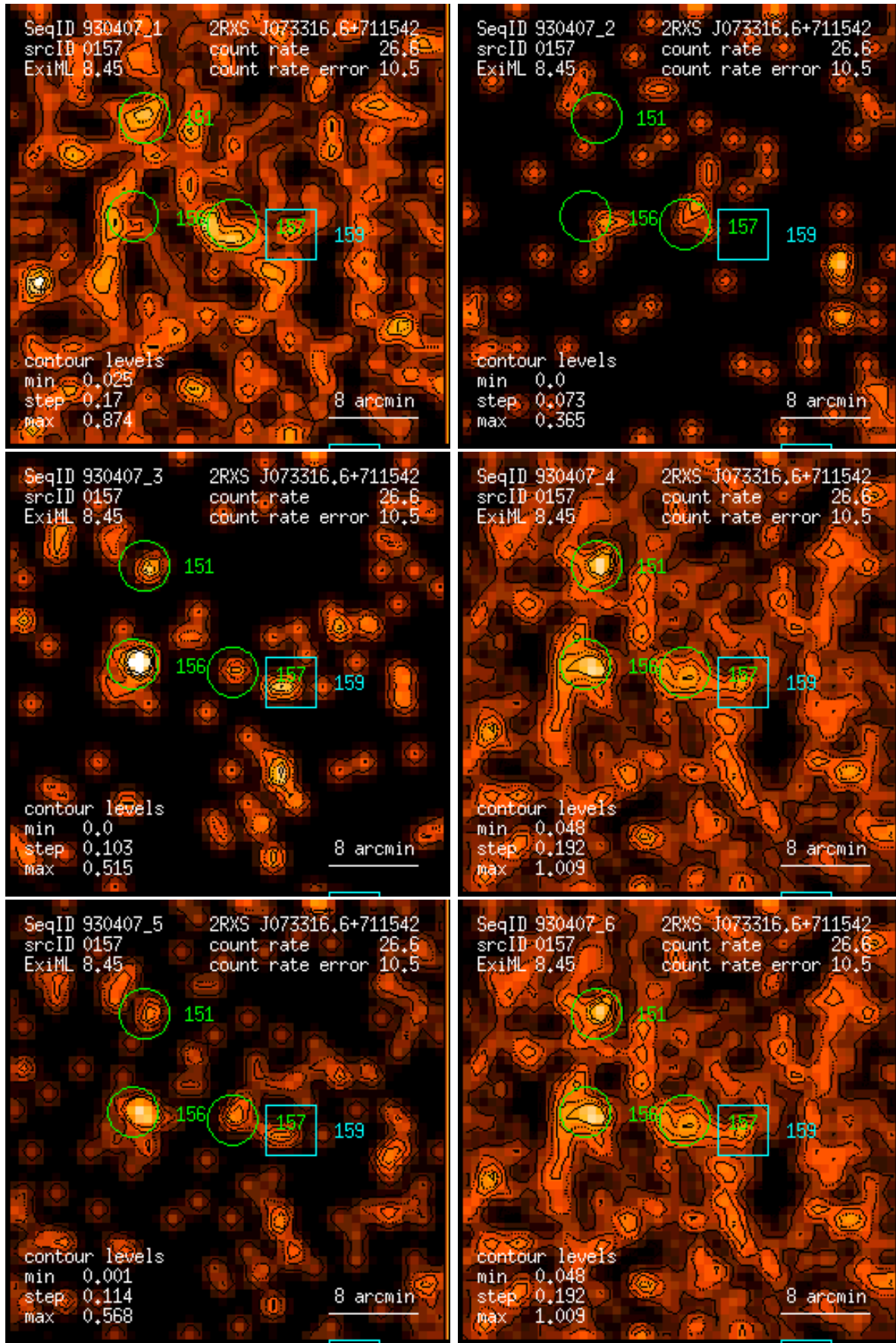
Figure 157: RASS 930407: detection 0157: band rate images, Gaussian filter: (1) PSPC channels 11 – 41, (2) 52 – 90, (3) 91 – 201, (4) 11 – 235, (5) 52 – 201, (6) 11 – 201. Broad band rates in counts/ks. Band rate contour levels in counts/ks/arcmin 2 .
