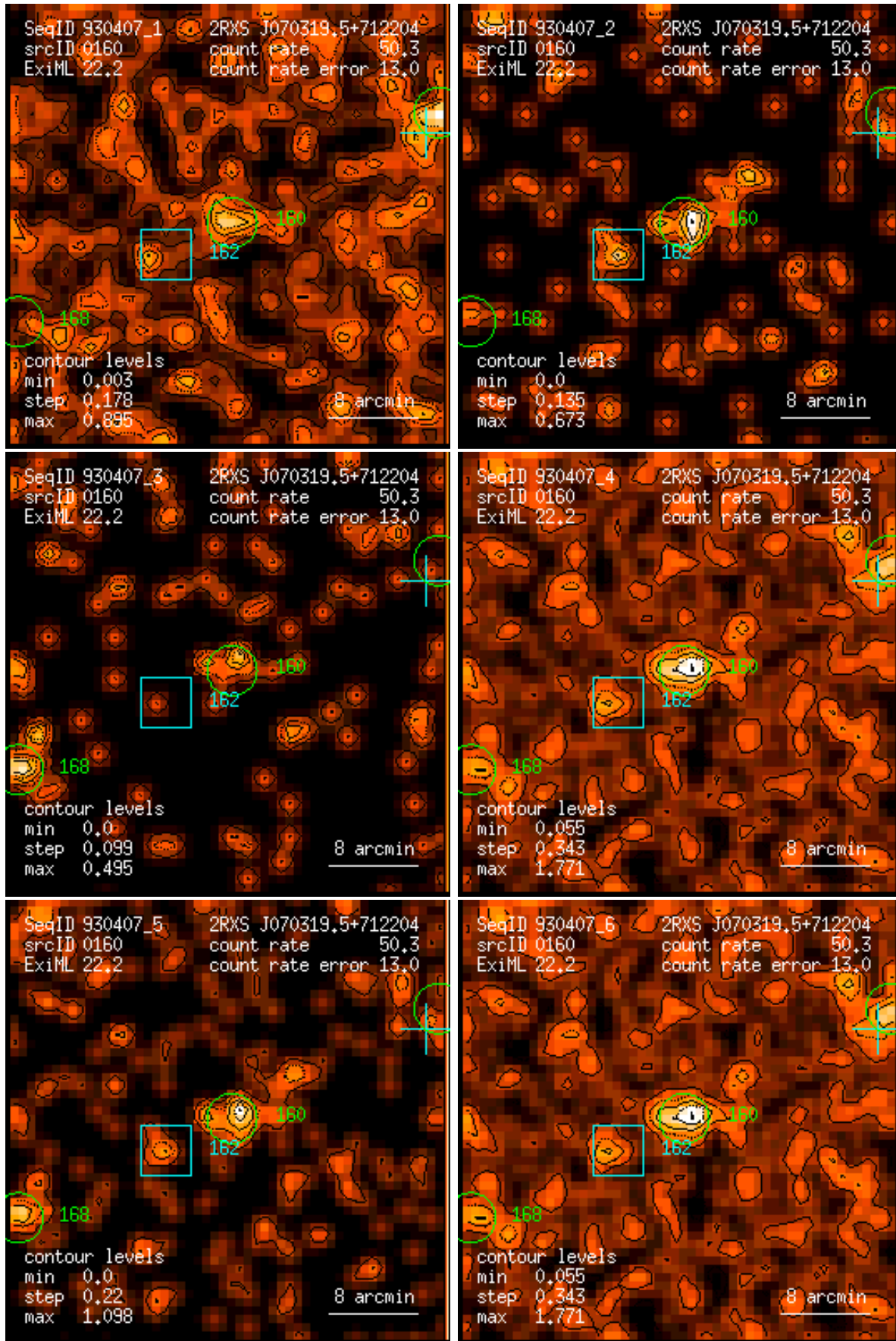
Figure 160: RASS 930407: detection 0160: band rate images, Gaussian filter: (1) PSPC channels 11 – 41, (2) 52 – 90, (3) 91 – 201, (4) 11 – 235, (5) 52 – 201, (6) 11 – 201. Broad band rates in counts/ks. Band rate contour levels in counts/ks/arcmin 2 .
