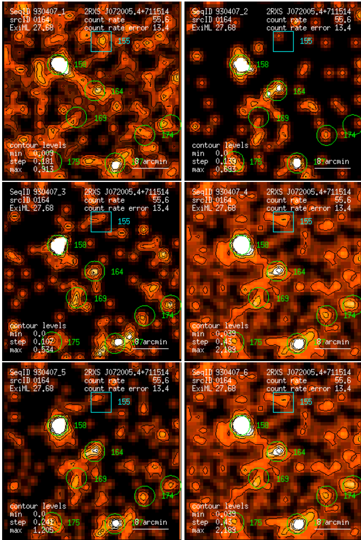
Figure 164: RASS 930407: detection 0164: band rate images, Gaussian filter: (1) PSPC channels 11 – 41, (2) 52 – 90, (3) 91 – 201, (4) 11 – 235, (5) 52 – 201, (6) 11 – 201. Broad band rates in counts/ks. Band rate contour levels in counts/ks/arcmin 2 .
