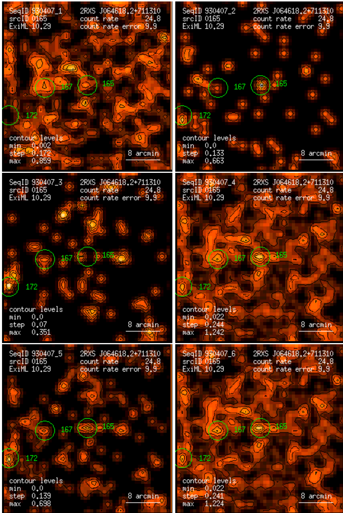
Figure 165: RASS 930407: detection 0165: band rate images, Gaussian filter: (1) PSPC channels 11 – 41, (2) 52 – 90, (3) 91 – 201, (4) 11 – 235, (5) 52 – 201, (6) 11 – 201. Broad band rates in counts/ks. Band rate contour levels in counts/ks/arcmin 2 .
