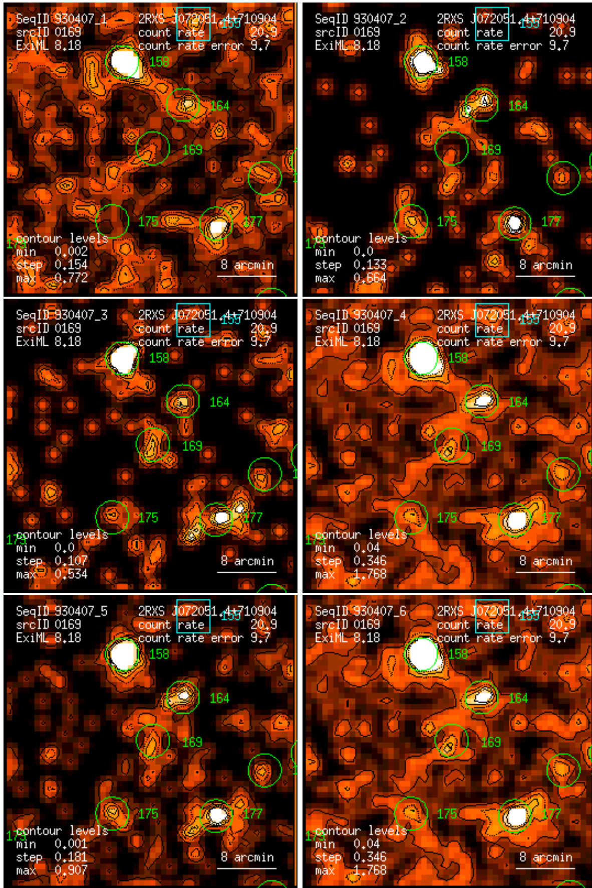
Figure 169: RASS 930407: detection 0169: band rate images, Gaussian filter: (1) PSPC channels 11 – 41, (2) 52 – 90, (3) 91 – 201, (4) 11 – 235, (5) 52 – 201, (6) 11 – 201. Broad band rates in counts/ks. Band rate contour levels in counts/ks/arcmin 2 .
