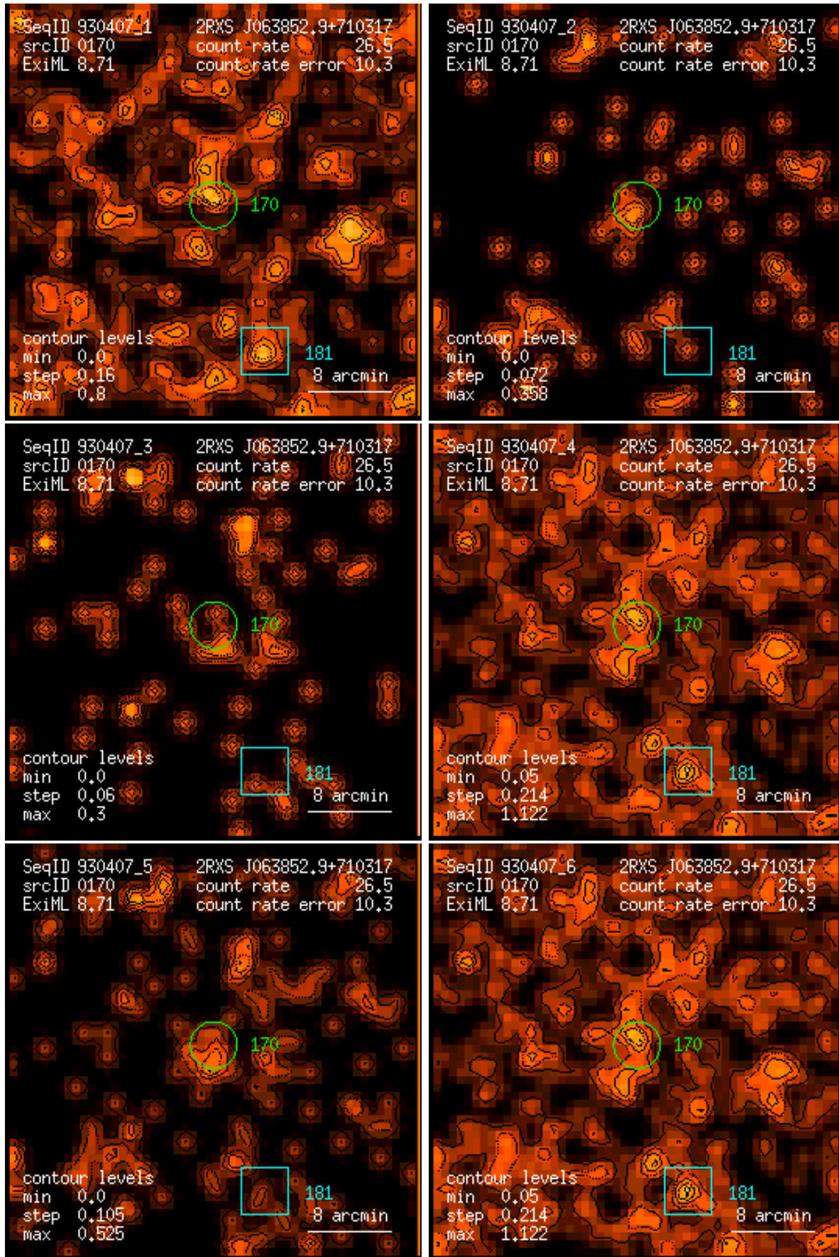
Figure 170: RASS 930407: detection 0170: band rate images, Gaussian filter: (1) PSPC channels 11 – 41, (2) 52 – 90, (3) 91 – 201, (4) 11 – 235, (5) 52 – 201, (6) 11 – 201. Broad band rates in counts/ks. Band rate contour levels in counts/ks/arcmin 2 .
