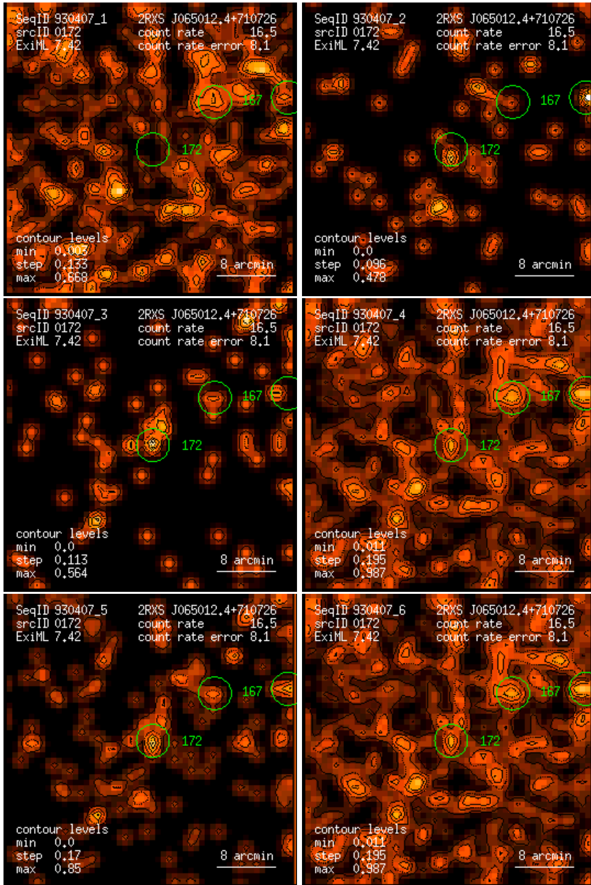
Figure 172: RASS 930407: detection 0172: band rate images, Gaussian filter: (1) PSPC channels 11 – 41, (2) 52 – 90, (3) 91 – 201, (4) 11 – 235, (5) 52 – 201, (6) 11 – 201. Broad band rates in counts/ks. Band rate contour levels in counts/ks/arcmin 2 .
