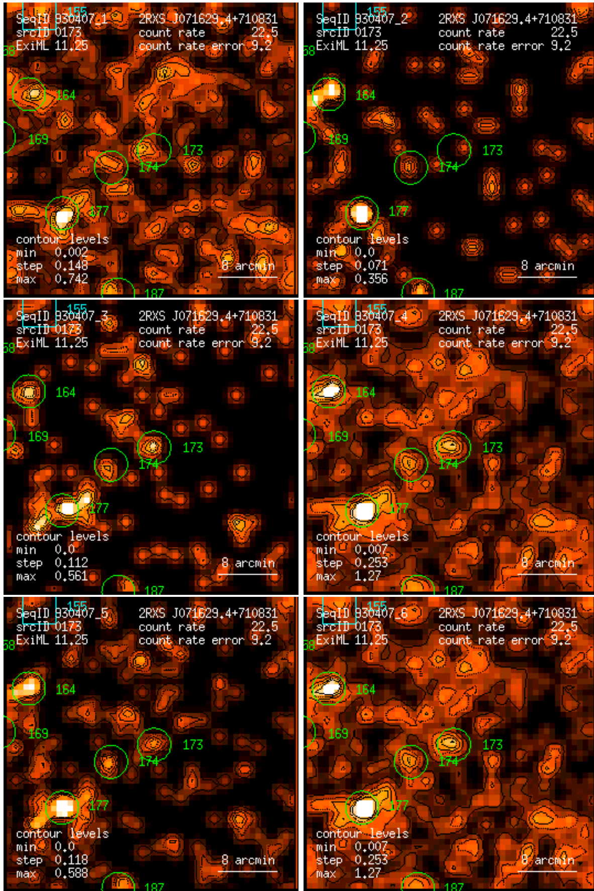
Figure 173: RASS 930407: detection 0173: band rate images, Gaussian filter: (1) PSPC channels 11 – 41, (2) 52 – 90, (3) 91 – 201, (4) 11 – 235, (5) 52 – 201, (6) 11 – 201. Broad band rates in counts/ks. Band rate contour levels in counts/ks/arcmin 2 .
