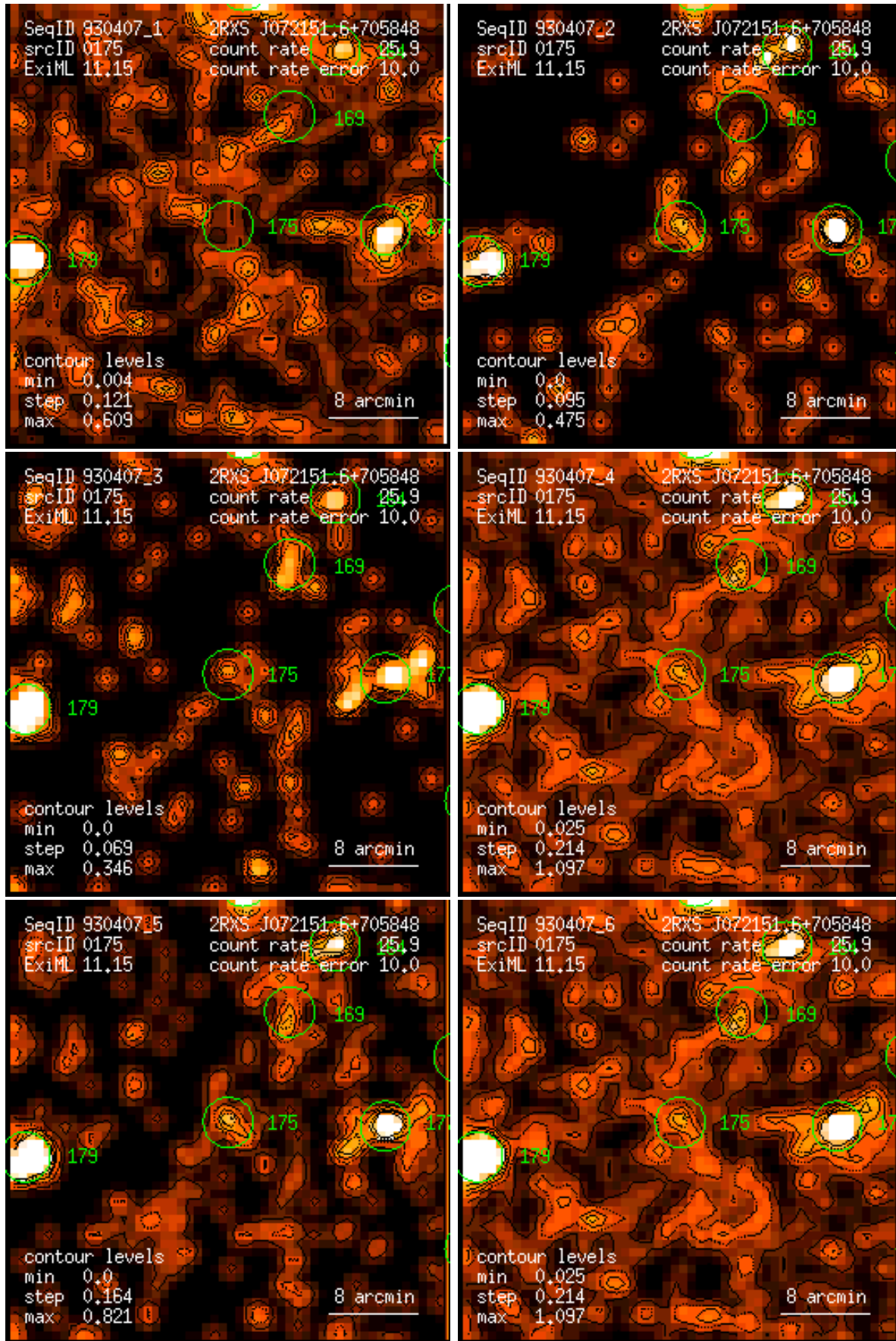
Figure 175: RASS 930407: detection 0175: band rate images, Gaussian filter: (1) PSPC channels 11 – 41, (2) 52 – 90, (3) 91 – 201, (4) 11 – 235, (5) 52 – 201, (6) 11 – 201. Broad band rates in counts/ks. Band rate contour levels in counts/ks/arcmin 2 .
