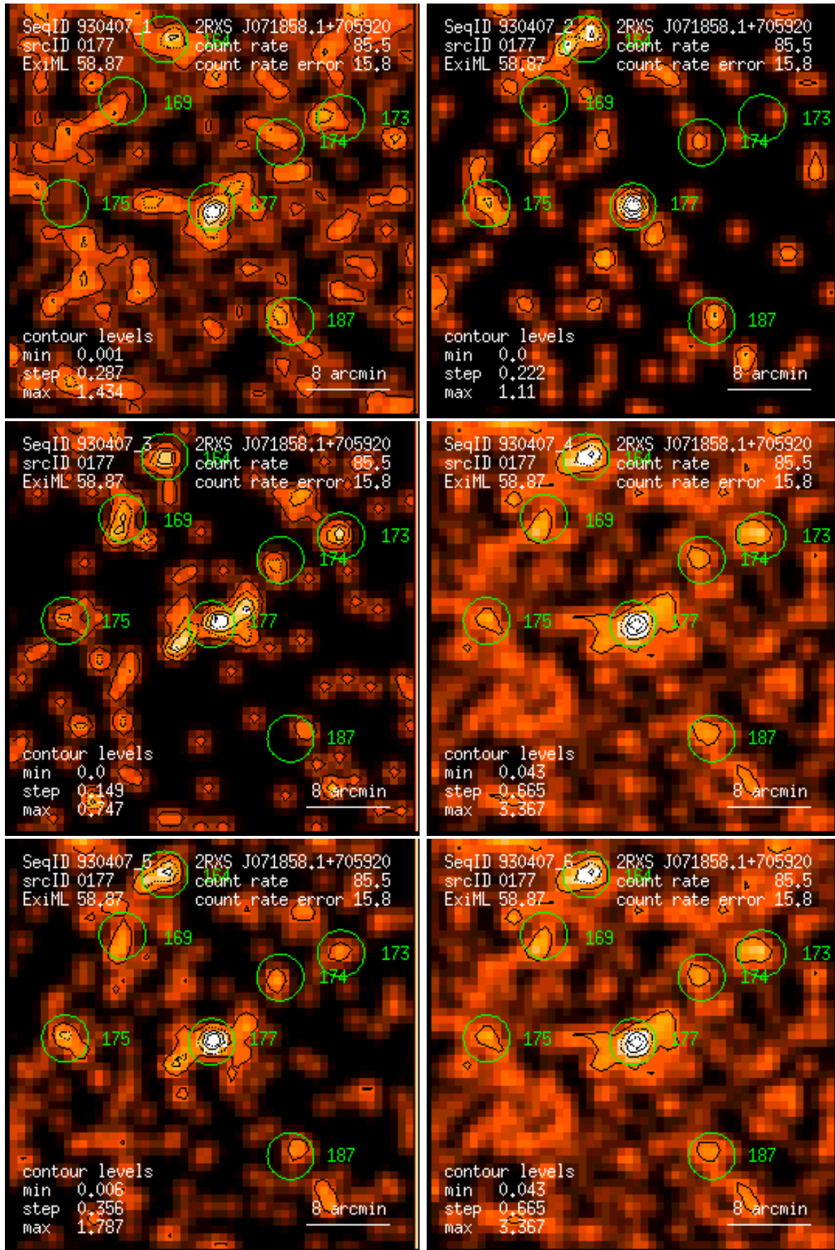
Figure 177: RASS 930407: detection 0177: band rate images, Gaussian filter: (1) PSPC channels 11 – 41, (2) 52 – 90, (3) 91 – 201, (4) 11 – 235, (5) 52 – 201, (6) 11 – 201. Broad band rates in counts/ks. Band rate contour levels in counts/ks/arcmin 2 .
