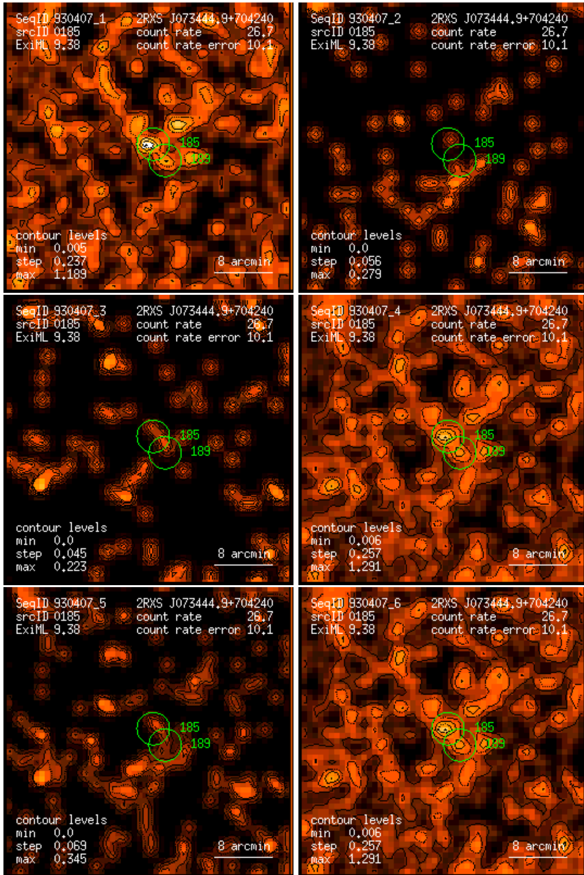
Figure 185: RASS 930407: detection 0185: band rate images, Gaussian filter: (1) PSPC channels 11 – 41, (2) 52 – 90, (3) 91 – 201, (4) 11 – 235, (5) 52 – 201, (6) 11 – 201. Broad band rates in counts/ks. Band rate contour levels in counts/ks/arcmin 2 .
