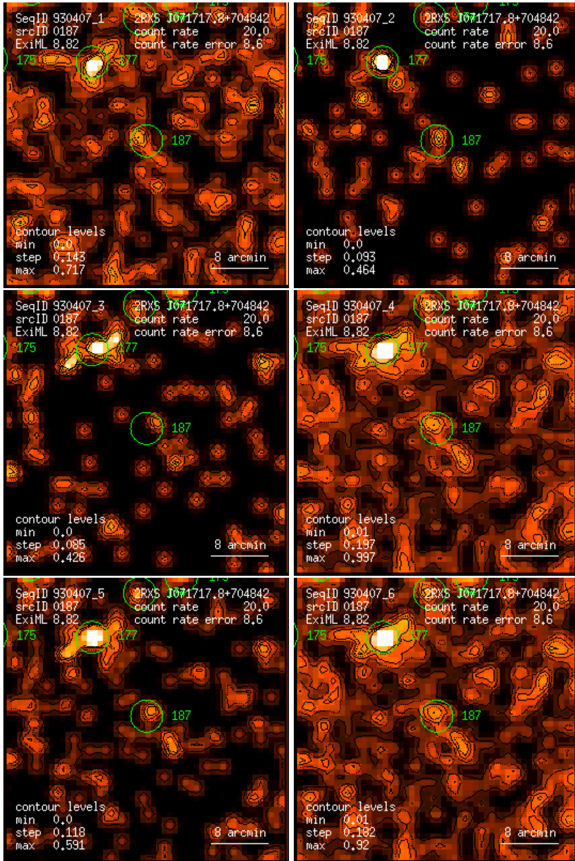
Figure 187: RASS 930407: detection 0187: band rate images, Gaussian filter: (1) PSPC channels 11 – 41, (2) 52 – 90, (3) 91 – 201, (4) 11 – 235, (5) 52 – 201, (6) 11 – 201. Broad band rates in counts/ks. Band rate contour levels in counts/ks/arcmin 2 .
