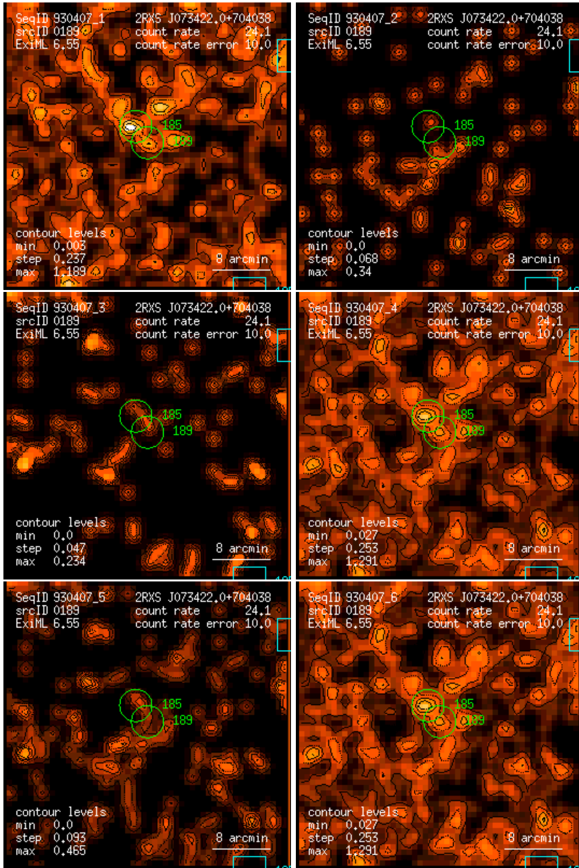
Figure 189: RASS 930407: detection 0189: band rate images, Gaussian filter: (1) PSPC channels 11 – 41, (2) 52 – 90, (3) 91 – 201, (4) 11 – 235, (5) 52 – 201, (6) 11 – 201. Broad band rates in counts/ks. Band rate contour levels in counts/ks/arcmin 2 .
