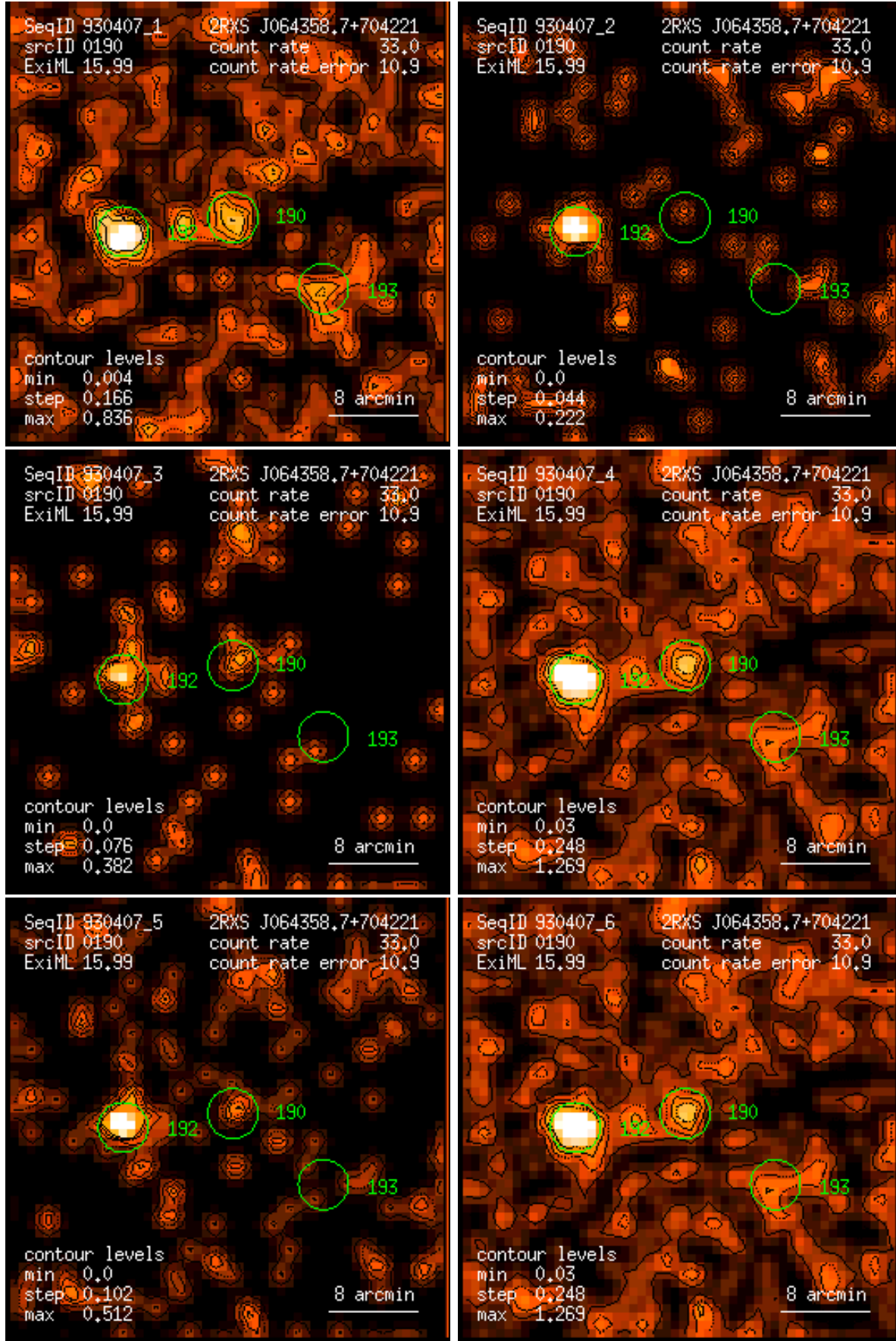
Figure 190: RASS 930407: detection 0190: band rate images, Gaussian filter: (1) PSPC channels 11 – 41, (2) 52 – 90, (3) 91 – 201, (4) 11 – 235, (5) 52 – 201, (6) 11 – 201. Broad band rates in counts/ks. Band rate contour levels in counts/ks/arcmin 2 .
