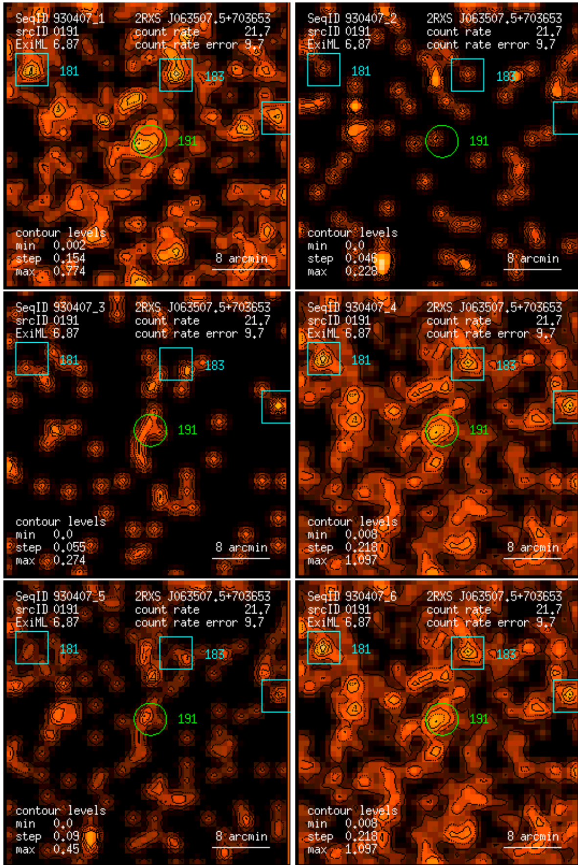
Figure 191: RASS 930407: detection 0191: band rate images, Gaussian filter: (1) PSPC channels 11 – 41, (2) 52 – 90, (3) 91 – 201, (4) 11 – 235, (5) 52 – 201, (6) 11 – 201. Broad band rates in counts/ks. Band rate contour levels in counts/ks/arcmin 2 .
