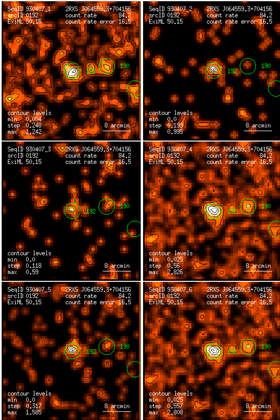
Figure 192: RASS 930407: detection 0192: band rate images, Gaussian filter: (1) PSPC channels 11 – 41, (2) 52 – 90, (3) 91 – 201, (4) 11 – 235, (5) 52 – 201, (6) 11 – 201. Broad band rates in counts/ks. Band rate contour levels in counts/ks/arcmin 2 .
