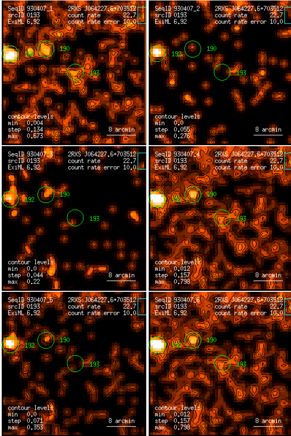
Figure 193: RASS 930407: detection 0193: band rate images, Gaussian filter: (1) PSPC channels 11 – 41, (2) 52 – 90, (3) 91 – 201, (4) 11 – 235, (5) 52 – 201, (6) 11 – 201. Broad band rates in counts/ks. Band rate contour levels in counts/ks/arcmin 2 .
