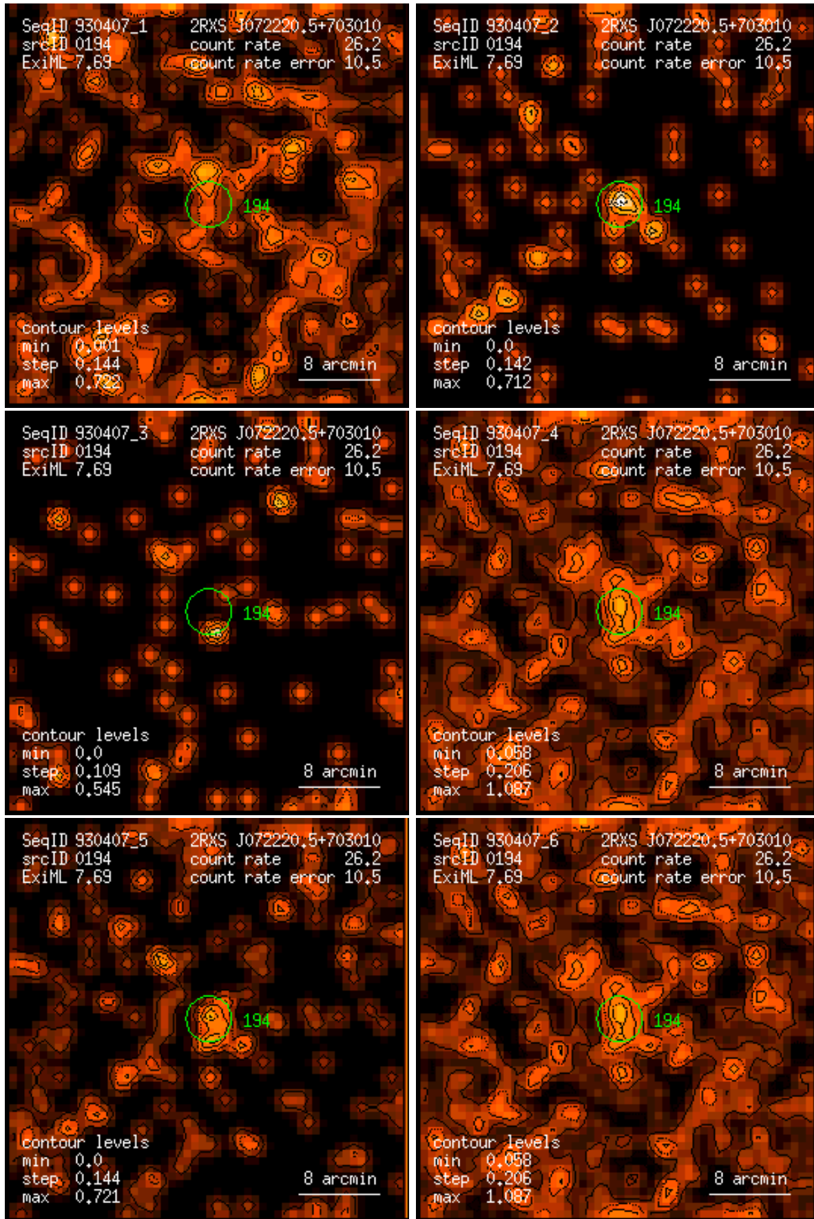
Figure 194: RASS 930407: detection 0194: band rate images, Gaussian filter: (1) PSPC channels 11 – 41, (2) 52 – 90, (3) 91 – 201, (4) 11 – 235, (5) 52 – 201, (6) 11 – 201. Broad band rates in counts/ks. Band rate contour levels in counts/ks/arcmin 2 .
