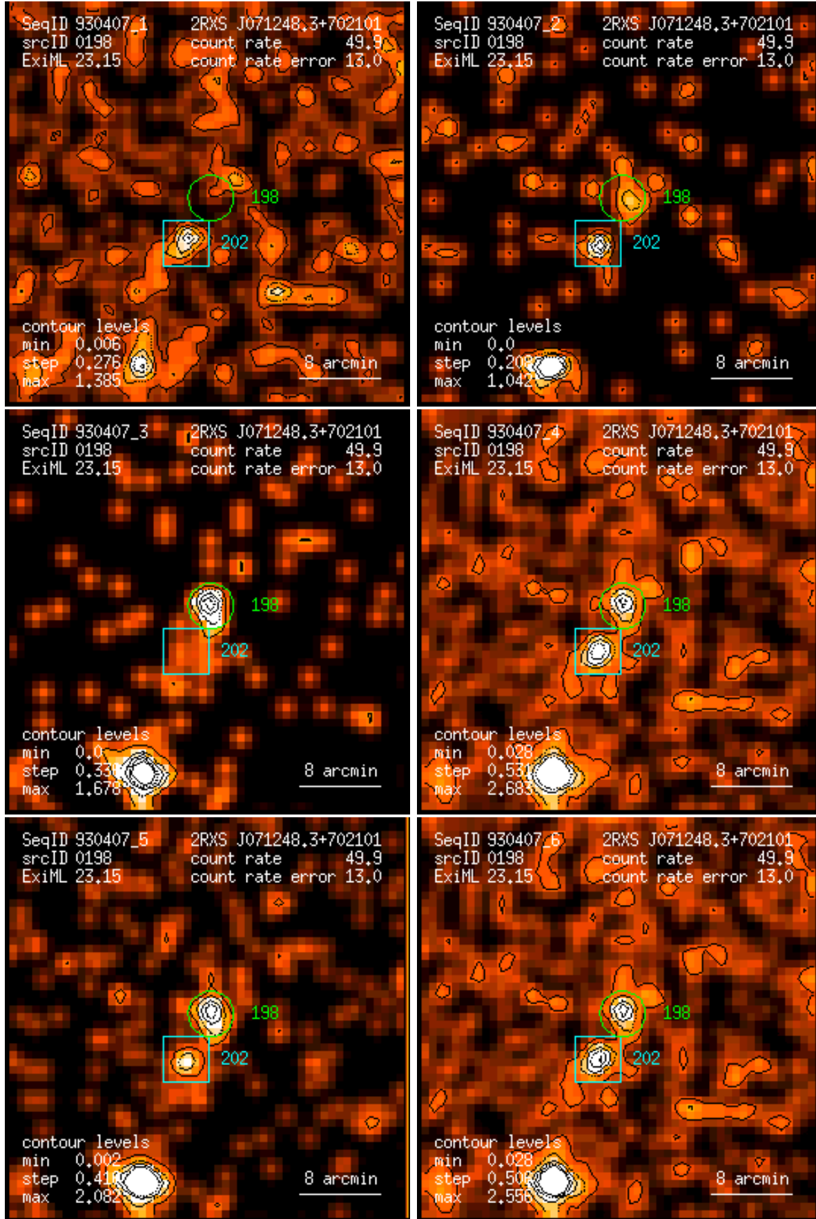
Figure 198: RASS 930407: detection 0198: band rate images, Gaussian filter: (1) PSPC channels 11 – 41, (2) 52 – 90, (3) 91 – 201, (4) 11 – 235, (5) 52 – 201, (6) 11 – 201. Broad band rates in counts/ks. Band rate contour levels in counts/ks/arcmin 2 .
