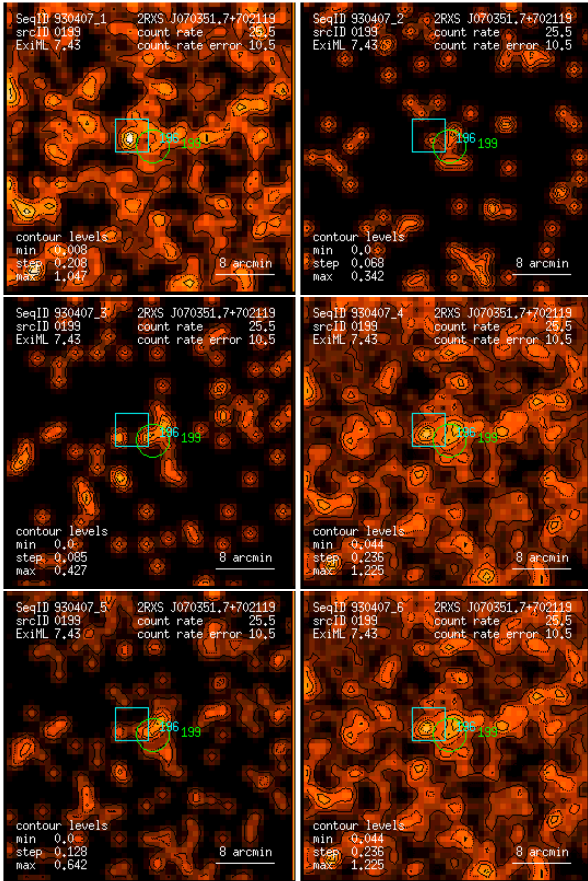
Figure 199: RASS 930407: detection 0199: band rate images, Gaussian filter: (1) PSPC channels 11 – 41, (2) 52 – 90, (3) 91 – 201, (4) 11 – 235, (5) 52 – 201, (6) 11 – 201. Broad band rates in counts/ks. Band rate contour levels in counts/ks/arcmin 2 .
